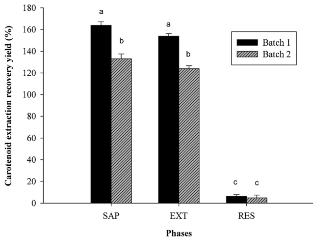
Fig. 5 Carotenoid recovery yields (%) of Nannochloropsis gaditana biomass (batches 1 and 2) extracted by using the improved method at the pilot scale after saponification (SAP), the extract fraction (EXT), and for the residual algal biomass (RES). Results are presented as the average \pm SD of two independent experiments. *Extraction recovery yield (% d.w.). Percentage of carotenoids extracted with respect to the compounds present in the initial biomass (batches 1 and 2) extracted by using the standard method (Cerón-García et al. 2018b) for the saponification step, the extraction, and the residue
