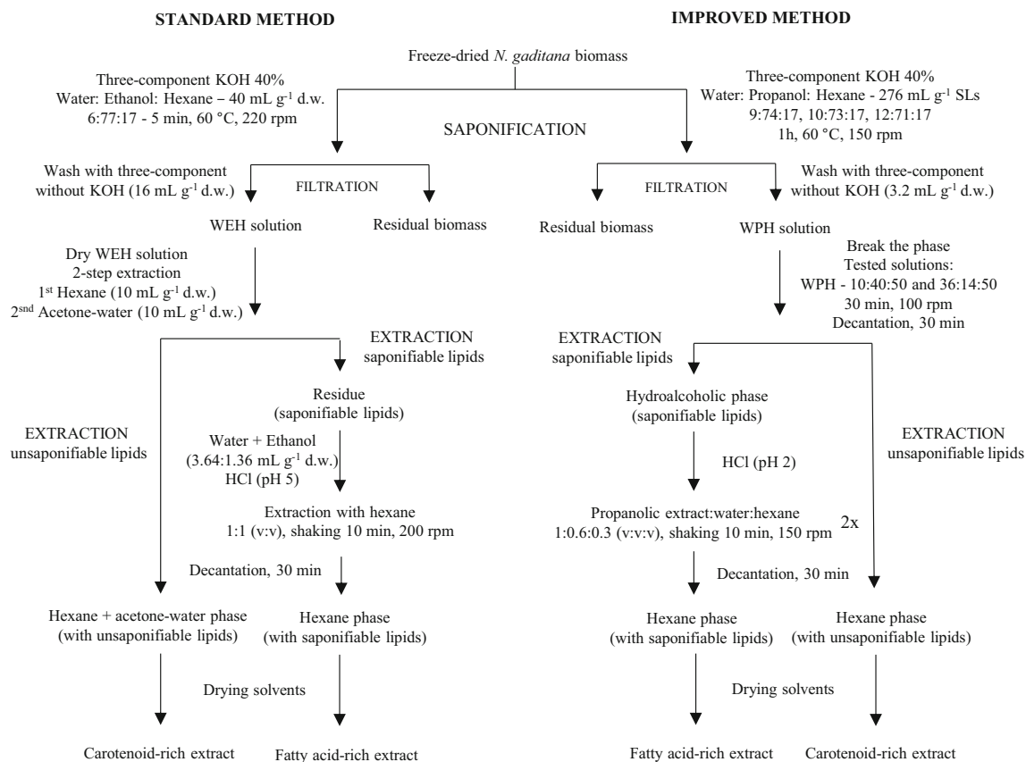
Fig. 1 Scheme of the extraction process for recovering carotenoids and fatty acids simultaneously from the Nannochloropsis gaditana microalga, a modification of the method proposed by Cerón-García et al. 2018b
