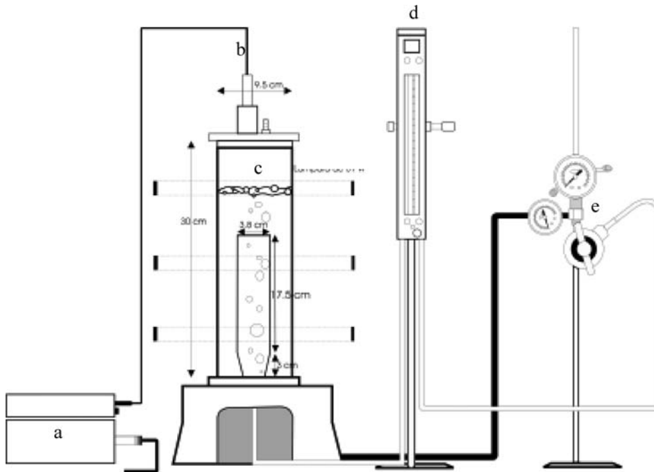
Fig. 1 Airlift bioreactor design. (a) Spectrophotometer, (b) Optic fiber, (c) Bioreactor, (d) Flow meter and (e) Manometer
