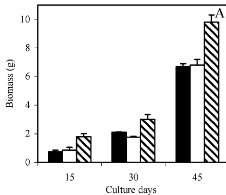
Fig. 5 A) Biomass increase of K. alvarezii explants after 15, 30 and 45 days cultivation in balloon flasks (black bars), airlift bioreactor (white bars) and Fernbach flasks (lined bars). B) Axes produced per explant in the three culture systems after 30 days cultivation. Explants cultured in vitro with plant growth
