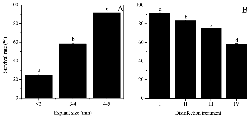
Fig. 2 K. alvarezii survival rate (%). A) Effect of explant size. B) Effect of disinfection treatment. I. Chlorine 1% 15 s + iodine 1% 15 s + antibiotics 24 h; II. Chlorine 1% 25 s + antibiotics 24
