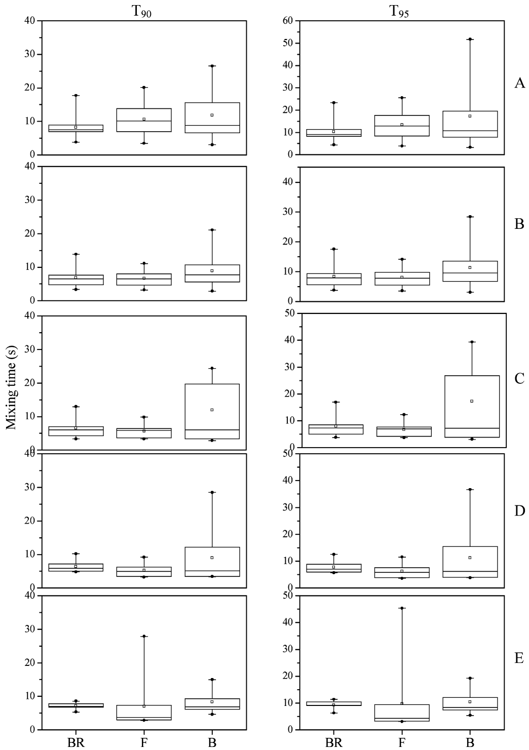
Fig. 6 Mixing times at T_{90} and T_{95} for airlift bioreactor (BR), Fernbach (F) and balloon flasks (B) at five working flow rates: (A) 200; (B) 400; (C) 600; (D) 800 and (E) 1000 mL min -1 ( \pm S.D.)
