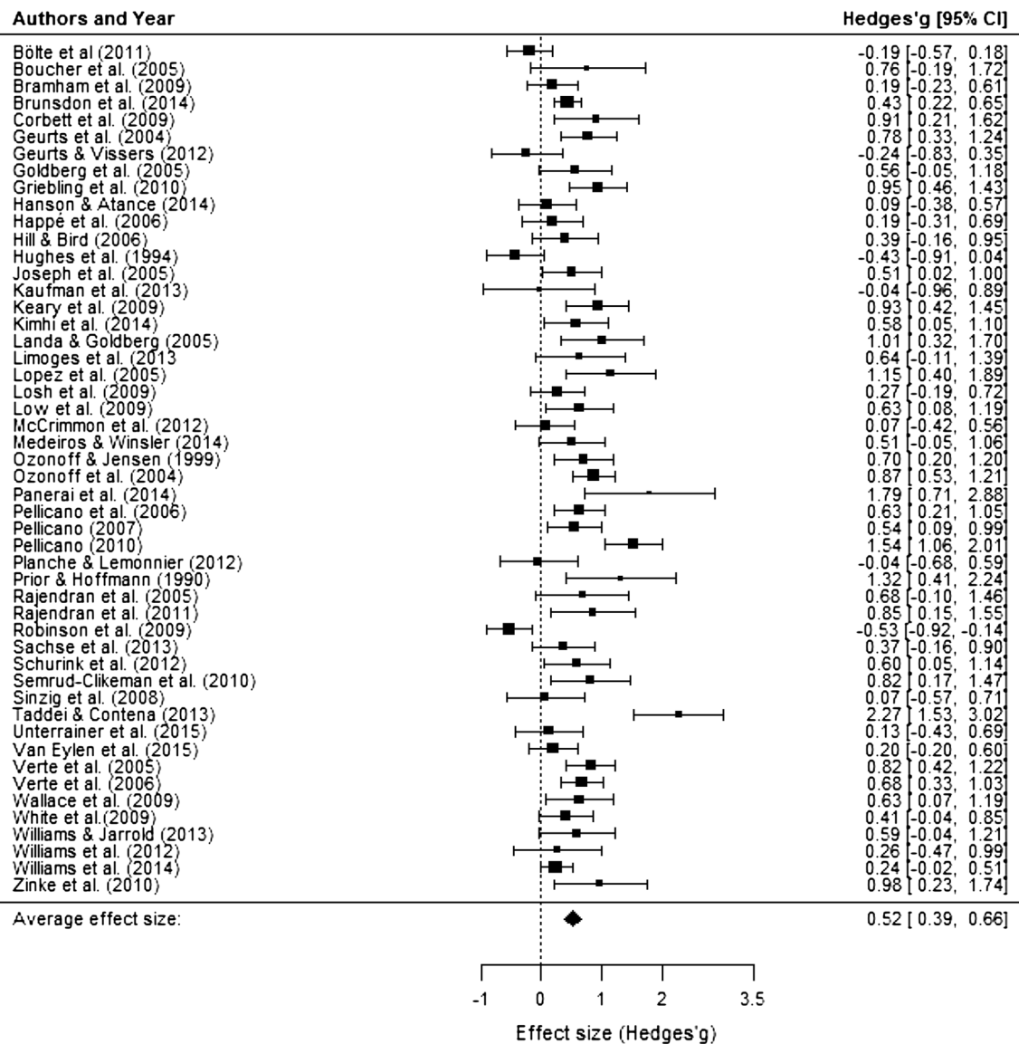
Fig. 2 Forest plot indicating effect sizes (Hedges' g) and 95% confidence intervals for each study effect included in the meta-analysis. Positive effect sizes indicate worse planning performance in the ASD
