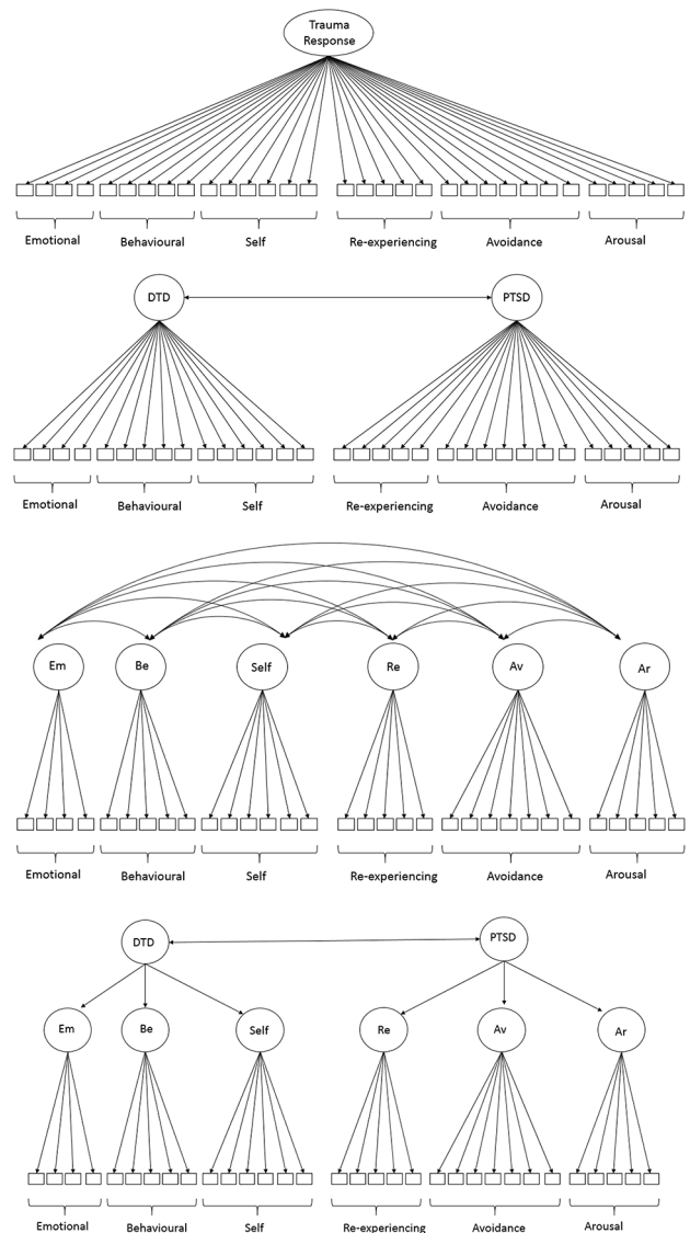
Fig. 1 Alternative Factor Models Model 1
