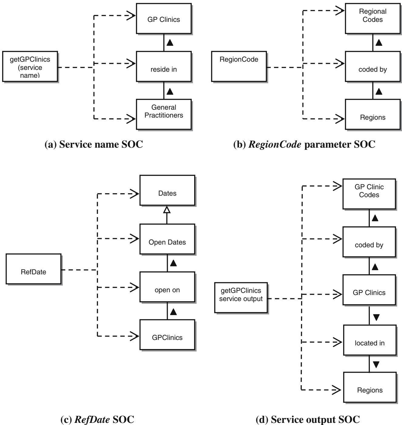
Fig. 3 Service Ontic Commitment (SOC) models of the getGPclinics web service
