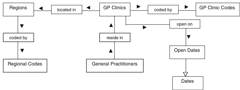
Fig. 4 First-cut domain model
