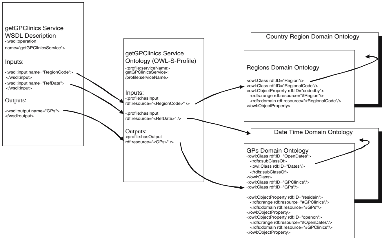
Fig. 6 Service-domain ontology topology
