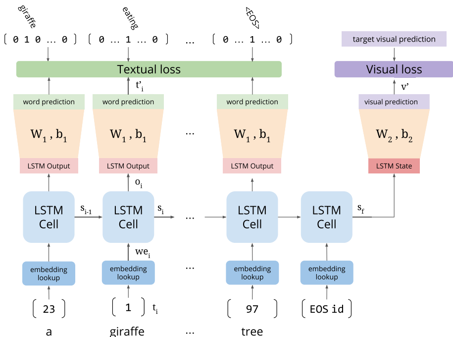
Fig. 3 Architecture of D-TEXT2VIS
