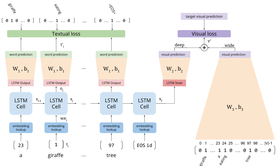
Fig. 4 Architecture of W&D-TEXT2VIS
