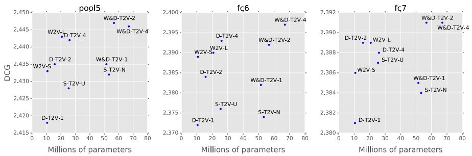
Fig. 6 Performance versus number of parameters to learn per model for all feature spaces (pool5, fc6, and fc7 from left to right). Prefix ‘S-’ denotes S-TEXT2VIS, ‘D-’ denotes D-TEXT2VIS, ‘W&D-’ denotes W&D-TEXT2VIS, and ‘W2V-’ denotes WORD2VISUALVEC
