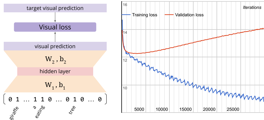
Fig. 1 Left: architecture of a simple regressor model with one hidden layer of size 1024. Right: the training and validation loss (on y-axis) in function of the training iteration (on x-axis). Notice the model overfits in the early phase of the training process
