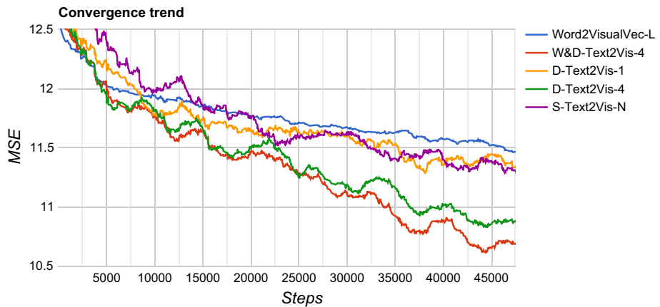
Fig. 7 Convergence error loss trends on the fc6 layer of some selected models
