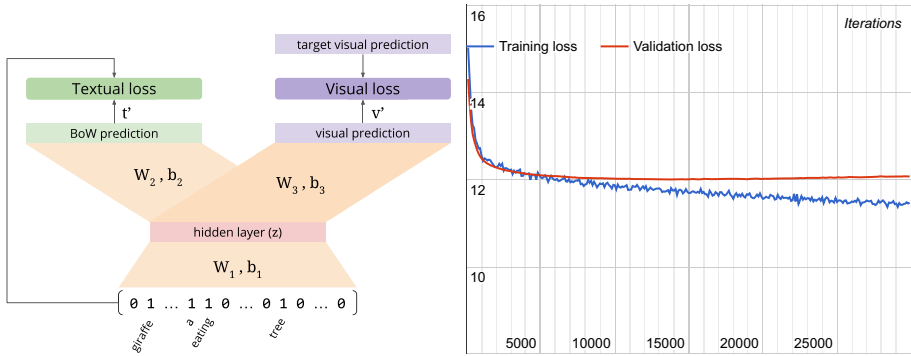
Fig. 2 Left: architecture of our proposed S-TEXT2VIS which controls overfitting by adding an autoencoding constraint on the hidden state. Right: the training and validation loss (on y-axis) in function of the training iteration (on x-axis)
