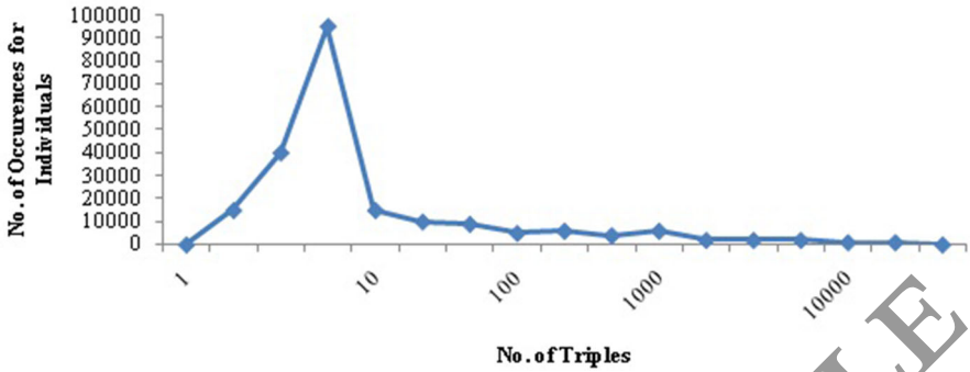
Fig. 8 Broadcasting triplets per individual’s occurrences
