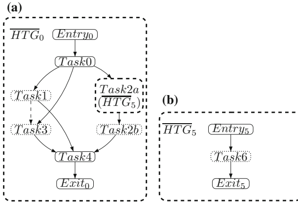
Fig. 7 \overline{HTG} created from HTG considering SolB. a Task Graph of L_0 . b Task Graph of L_5
