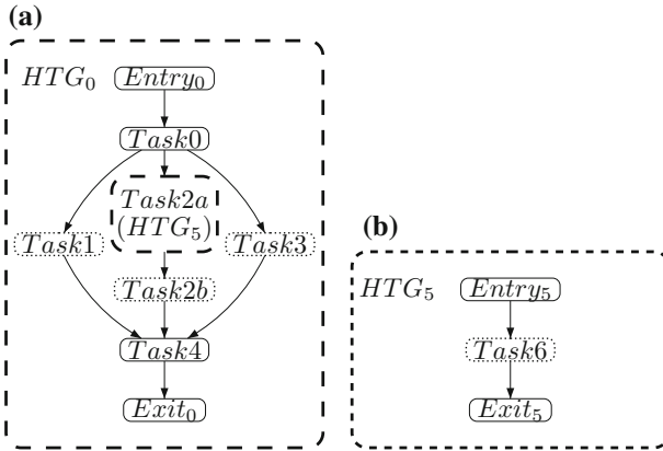
Fig. 5 Hierarchical Task Graph extracted from function fun_0 . a Task Graph of L_0 . b Task Graph of L_5
