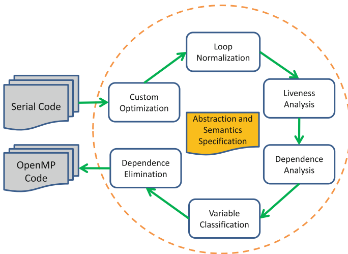
Fig. 5 A semantic-aware parallelizer built using ROSE
