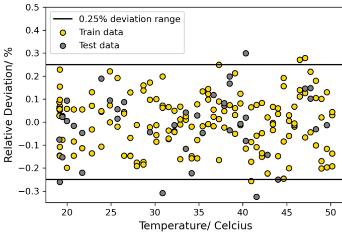
Fig. 14 The variation of relative deviation of viscosity ANN model with temperature
