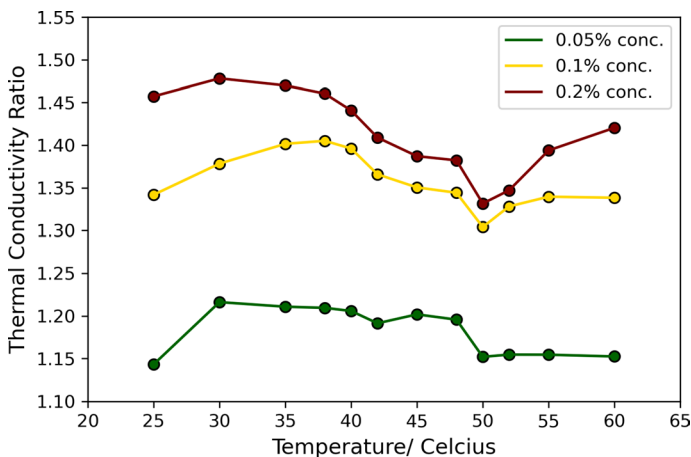
Fig. 4 Thermal conductivity ratio variation with temperature for various concentrations
