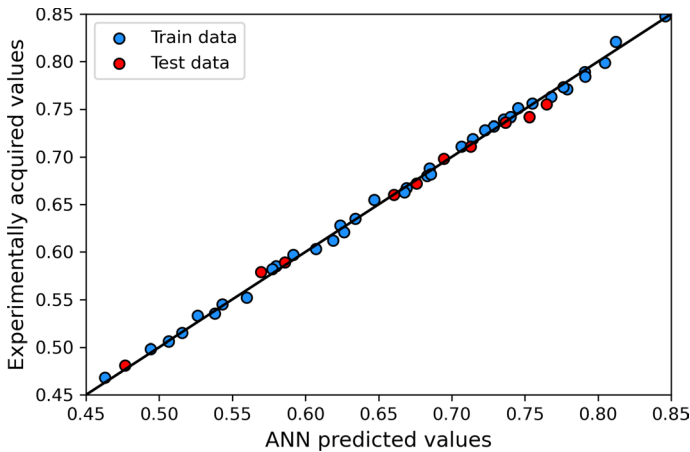
Fig. 8 Comparison between experimentally acquired thermal conductivity values and their ANN predictions
