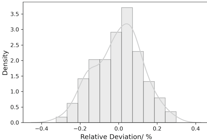
Fig. 16 The histogram of the relative deviation of viscosity ANN model
