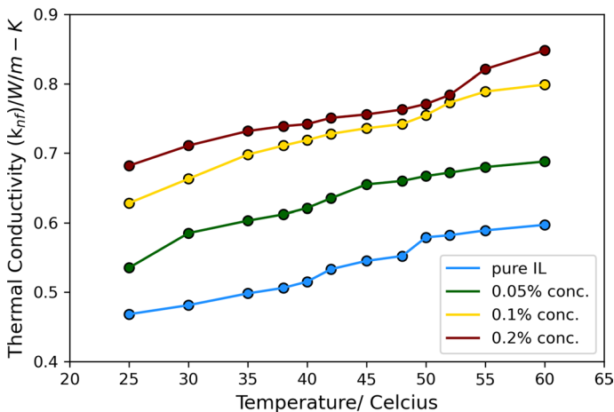
Fig. 3 Thermal conductivity of aqueous IoNanofluid for various temperatures and concentrations
