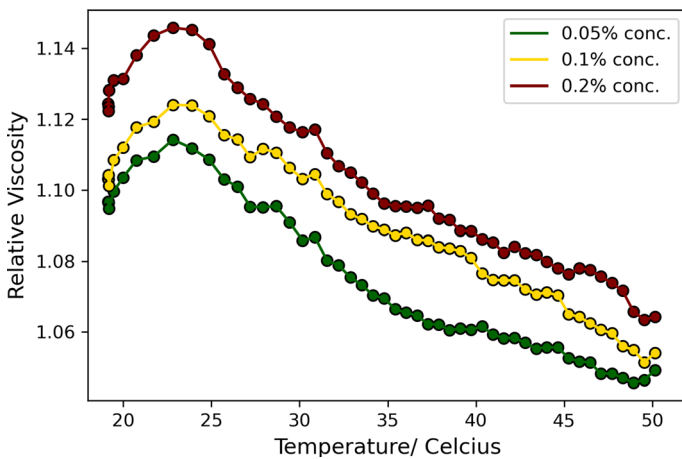
Fig. 6 Relative viscosity variation with temperature for various concentrations
