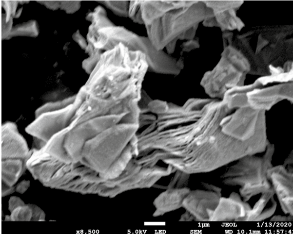
Fig. 1 FESEM analysis of the synthesized MXene nanomaterials at 1 \mu\text{m} magnification
