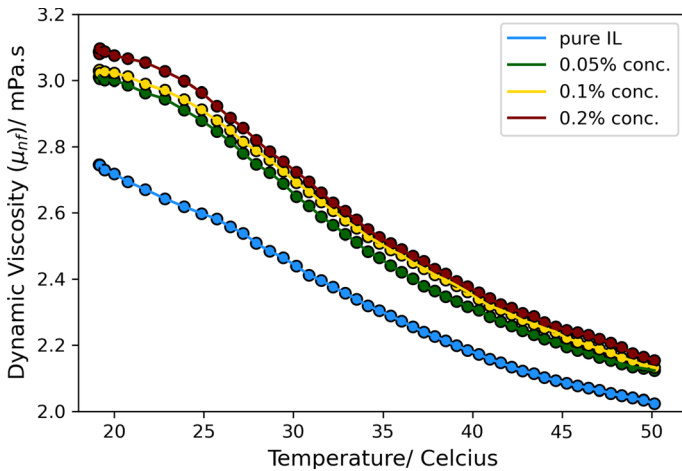
Fig. 5 Viscosity variation with temperature for various concentrations
