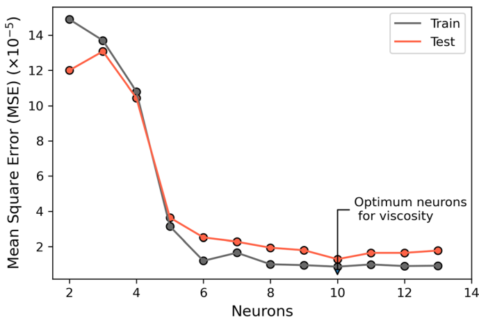
Fig. 12 Variation of mean square error with number of neurons in hidden layer for viscosity model
