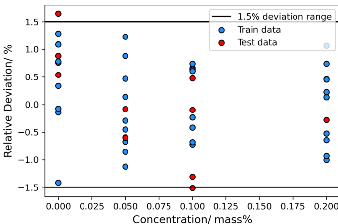
Fig. 10 The variation of relative deviation of thermal conductivity ANN model with MXene concentration
