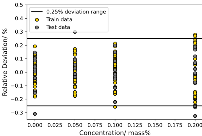
Fig. 15 The variation of relative deviation of viscosity ANN model with MXene concentration
