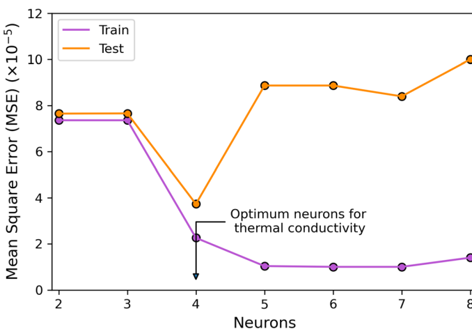
Fig. 7 Variation of mean square error with number of neurons in hidden layer for thermal conductivity model
