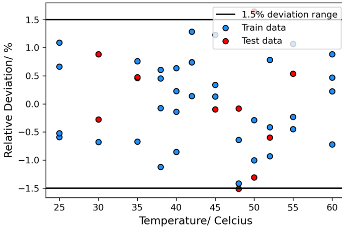
Fig. 9 The variation of relative deviation of thermal conductivity ANN model with temperature
