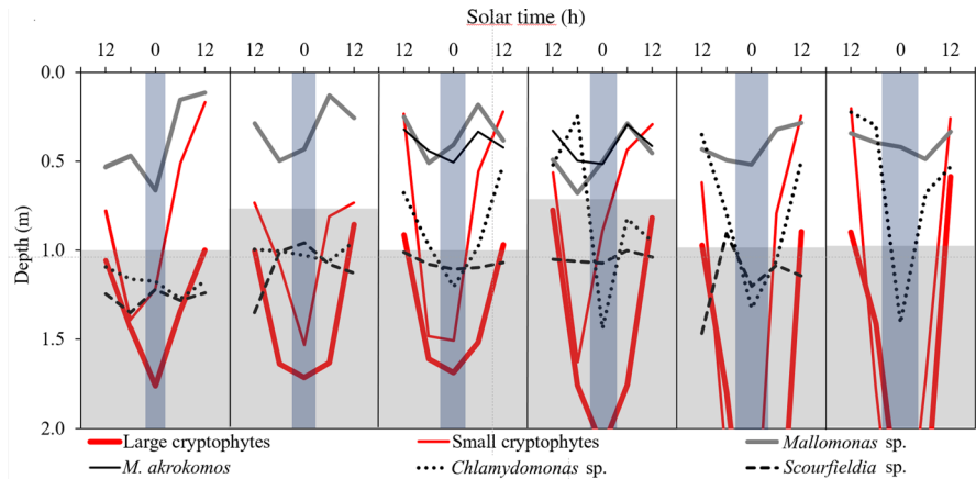
Fig. 7 The median diel vertical positions of motile phytoplankton species at 6 h (solar time) intervals on the sampling days. Bottom grey area—anoxic zone; vertical dark shaded bars—periods between sunset and sunrise; because the two uppermost samples of the first sampling day were lost, the broken lines (except for Scourfieldia sp.) underestimate the height of the median position at the first noon
