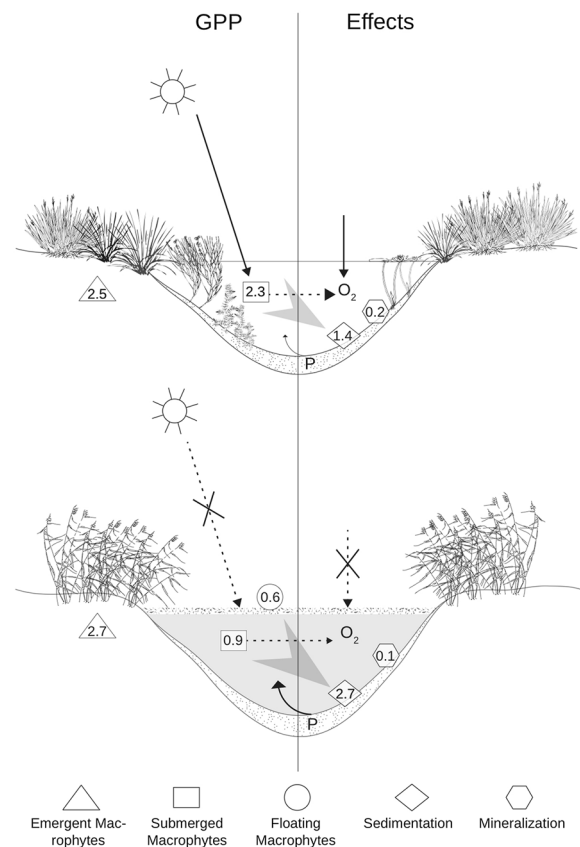
Fig. 5 Gross primary production (GPP) of the different primary producer groups during peak summer months (June to August) and their cascading effects on phosphorus (P) release from sediments and carbon sediment deposition and mineralisation (all units in \text{g C m}^{-2} \text{day}^{-1} ) in A Kraatz and B Rittgarten. Phytoplankton and periphyton constituted <10% of community GPP in the summer and hence were not shown here. Triangles represent emergent macrophyte GPP, rectangles represent submerged macrophyte GPP and circles depict floating macrophyte GPP
