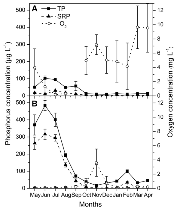
Fig. 1 Temporal fluctuations of total phosphorus (TP), soluble reactive phosphorus (SRP) concentrations ( \mu\text{g l}^{-1} ) and oxygen concentrations ( \text{mg l}^{-1} ) throughout the sampling period (May 2013 to April 2014) in two kettle holes A Kraatz and B Rittgarten
