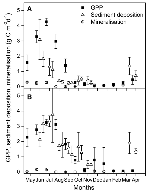
Fig. 3 Temporal variations of total gross primary production (GPP), sediment deposition rates and sediment aerobic mineralisation rates in two kettle holes: A Kraatz and B Rittgarten from May 2013 to April 2014
