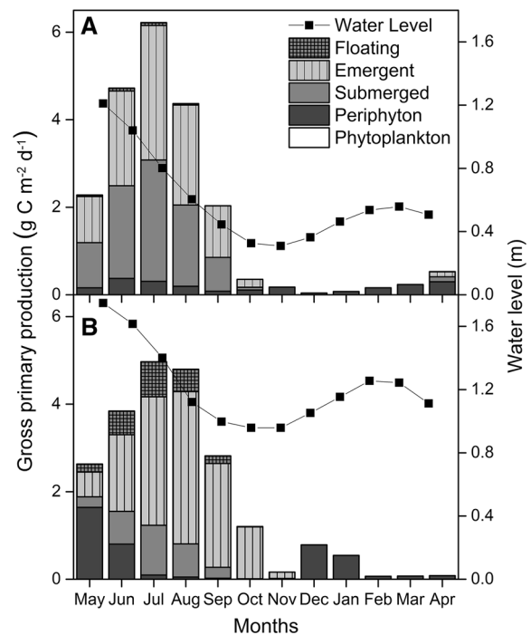
Fig. 2 Monthly gross primary production (GPP, \text{g C m}^{-2} \text{ day}^{-1} ) including the contributions of different primary producer groups in two kettle holes: A Kraatz B Rittgarten
