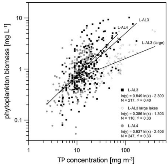
Fig. 2 Regression analysis between annual mean total phosphorus concentration and annual mean phytoplankton biomass (biovolume) in lakes belonging to the Alpine lake types L-AL3 and L-AL4. Regressions are calculated separately for L-AL3, very large lakes of L-AL3 (mean depth >100 m) and L-AL4
