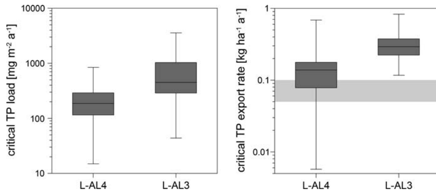
Fig. 1 Critical total phosphorus (TP) load per lake area after Vollenweider ( \text{mg m}^{-2} \text{a}^{-1} ) (left) and critical TP export rate from the catchment area ( \text{kg ha}^{-1} \text{a}^{-1} ) in the Alpine lake types L-AL3 (mean depth >15 m) and L-AL4 (mean depth 3–15 m,
