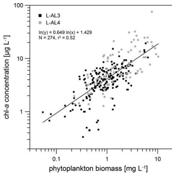
Fig. 3 Regression analysis between annual mean phytoplankton biomass (biovolume) and annual mean chlorophyll- a concentration in lakes belonging to the Alpine lake types L-AL3 and L-AL4. Very large and deep lakes of L-AL3 are not calculated separately
