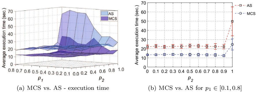
Fig. 4 The average execution time of MCS and AS algorithms
