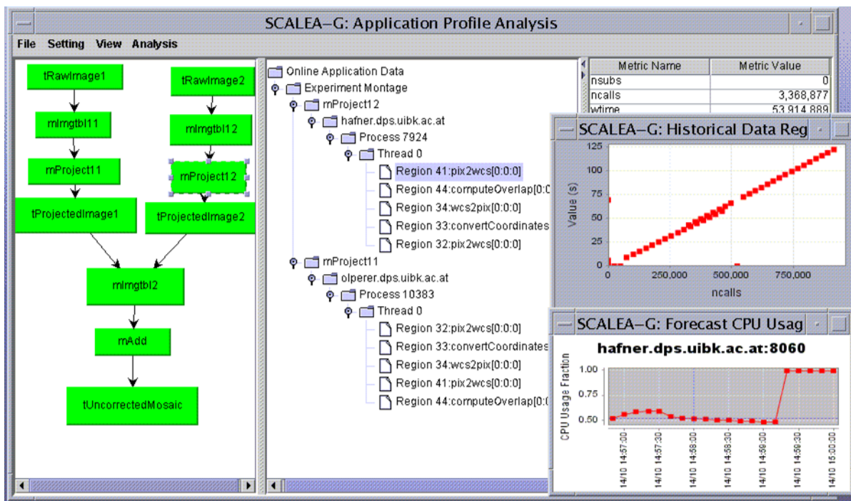
Figure 11. Performance analysis of workflow activities.
