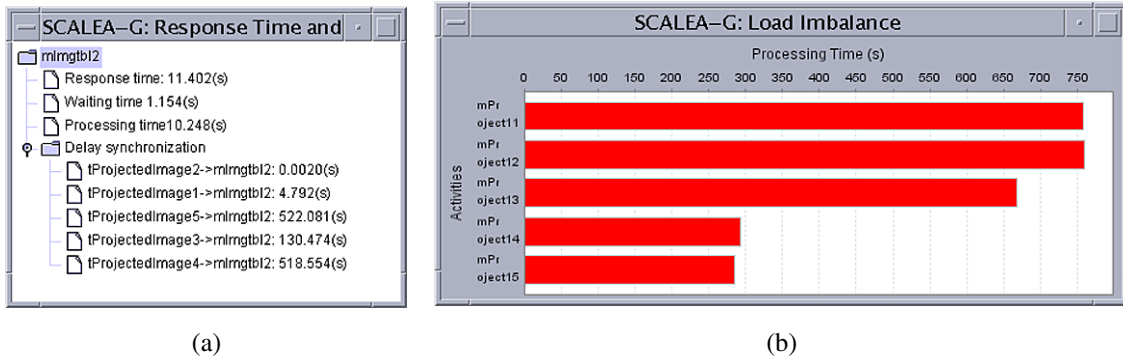
Figure 12. Analysis of Montage executed on 5 machines: (a) response time and synchronization delay of mImgtb1, and (b) load imbalance of mProject.
