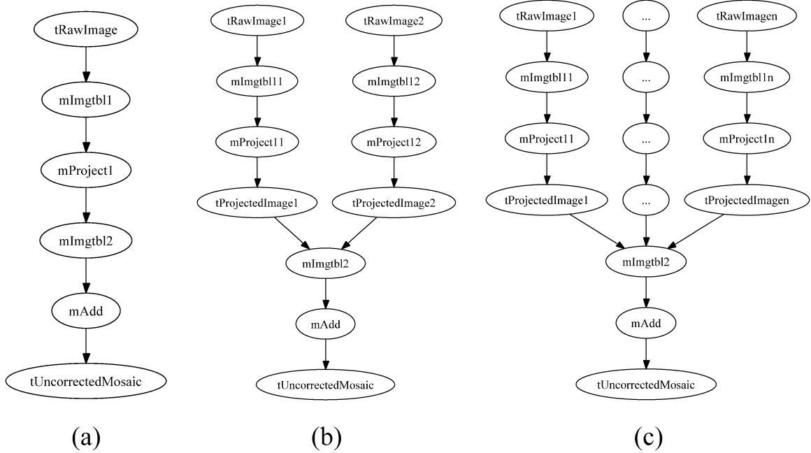
Figure 7. Experimental workflows of the Montage application: (a) workflow executed on single resource, (b) workflow executed on two resources, and (c) workflow executed on n resources.
