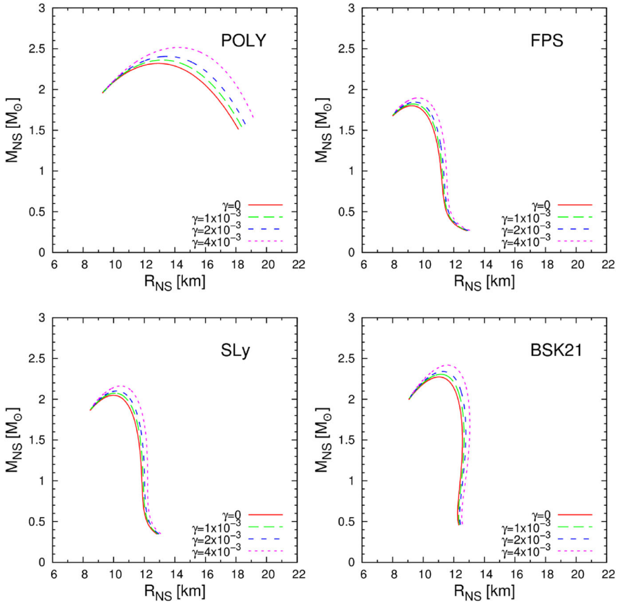
Fig. 1 Mass-radius relations for neutron star models with central densities in the range: 14.6 < \log(\rho_c [\text{g cm}^{-3}]) < 15.9 . We consider four different EoS: POLY ( top, left ), FPS ( top, right ), Sly ( bottom, left ) and BSK21 ( bottom, right ). The parameter \gamma quantifies the deviation of STVG from GR. In particular, \gamma = 0 corresponds to GR predictions. As we can see, greater \gamma implies higher maxima for neutron star total masses
