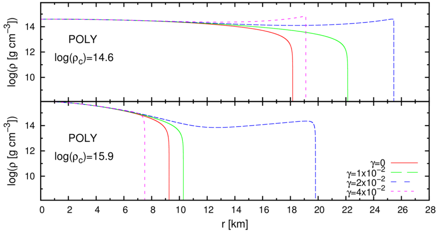
Fig. 4 Density profiles for POLY neutron star models with central densities: \log(\rho_c [\text{g cm}^{-3}]) = 14.6 (up) and \log(\rho_c [\text{g cm}^{-3}]) = 15.9 (down). Significant differences between STVG and GR predictions arise from \gamma \propto 10^{-2} . Repulsive gravity effects are intensified in low density models, up to a certain limit, when enhanced attraction prevails. High density neutron star profiles show similar features but, enhanced attraction effects take place at smaller radii
