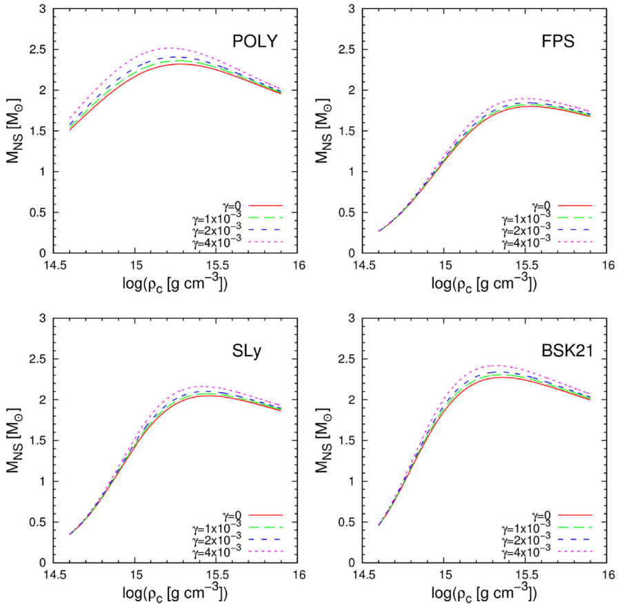
Fig. 2 Relation between neutron star total masses and their central densities. As mentioned, the parameter \gamma quantifies the deviation of STVG from GR. We consider four different EoS: POLY (top, left), FPS (top, right), Sly (bottom, left) and BSK21 (bottom, right). We find that the highest masses for STVG are achieved for lower central densities than in GR
