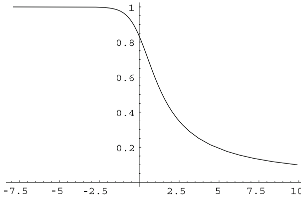
Fig. 2 The Hubble parameter as a function of time ( \sigma = 1 )
