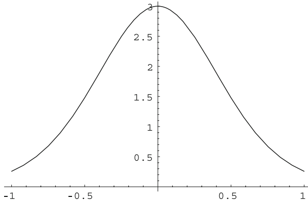
Fig. 1 The scalar field potential corresponding to Eq. (4) as a function of \phi (\sigma = 1)
