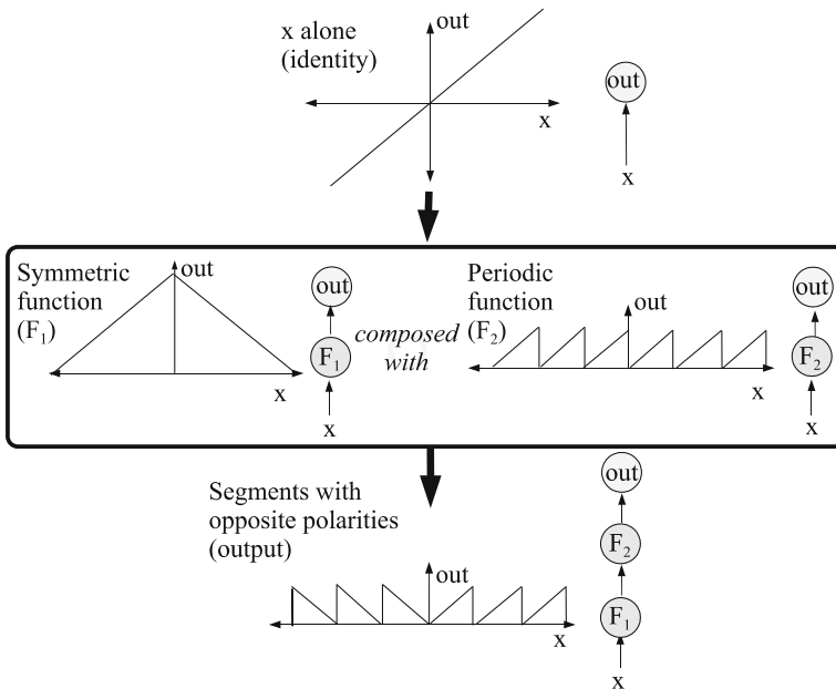
Fig. 3 Composing gradient functions. This example illustrates how a simple composition of functions in one dimension can produce a pattern with multiple regularities. A network representation of each composition is depicted to the right of each function graph. The initial asymmetric gradient x is composed with both a symmetric function ( F_1 ) and a periodic function ( F_2 ), resulting in two sets of segments with opposite polarity. Thus, new coordinate frames can be built upon preexisting ones without local interaction
