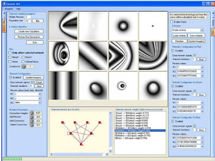
(b) SharpNEAT-based Genetic Art (SNGA)
