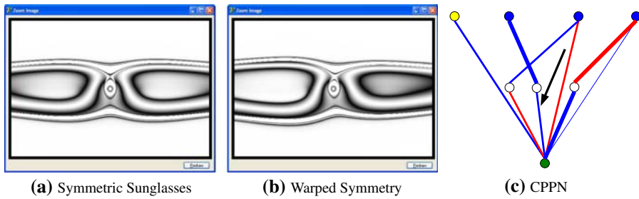
Fig. 9 Varying symmetry. A single connection gene controls the level of symmetry in the pattern. (a) The original pattern displays perfect bilateral symmetry. (b) By manipulating a single gene, the symmetry can be varied, yet without breaking the overall regularity of the structure. (c) An arrow points to the single gene responsible for asymmetry. Since overall regularity is preserved, the representation of the sunglasses by the CPPN cannot be strictly hierarchical
