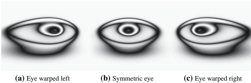
Fig. 10 Eye asymmetries. The eye-generating CPPN can produce all three eyes above by varying only one connection weight. Interestingly, the eye turns as if in a three-dimensional space, showing that the composition of functions can result in complex new coordinate frames, sometimes having meaningful real-world interpretations, such as rotational variance in a three-dimensional space
