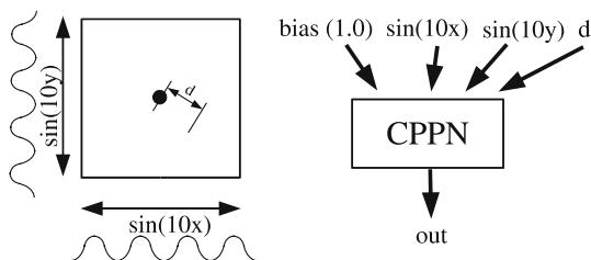
Fig. 11 CPPN periodic inputs. Instead of inputting x and y as usual, \sin(10x) and \sin(10y) are input in the experiments in Sect. 4.4. These inputs create a novel, repeating coordinate frame on which the CPPN can now elaborate. The purpose of this experiment is to show the powerful effect that coordinate transformation can have on phenotypic patterning
