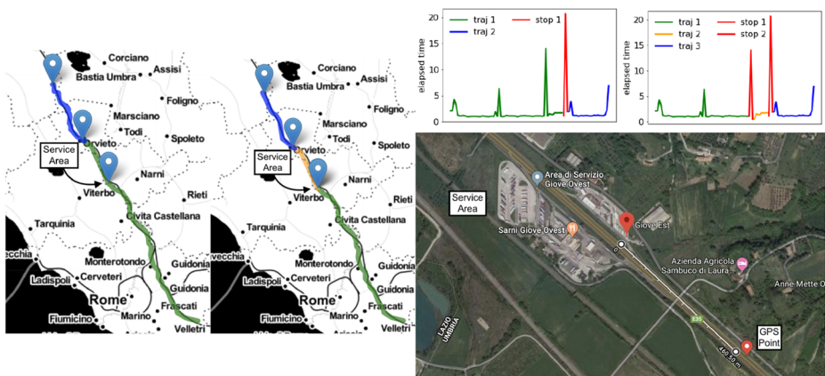
Fig. 7 Trajectory segmentation returned by FTS_{1200} (left) and ATS (right). The user is traveling from South to North. Top : spatial representation showing the trajectory segments. Center : temporal segmentation showing the inter-leaving time between GPS points. Bottom : zoom on the service area highlighted in the top maps where the user probably stops for ~ 15 minutes. Best viewed in color
