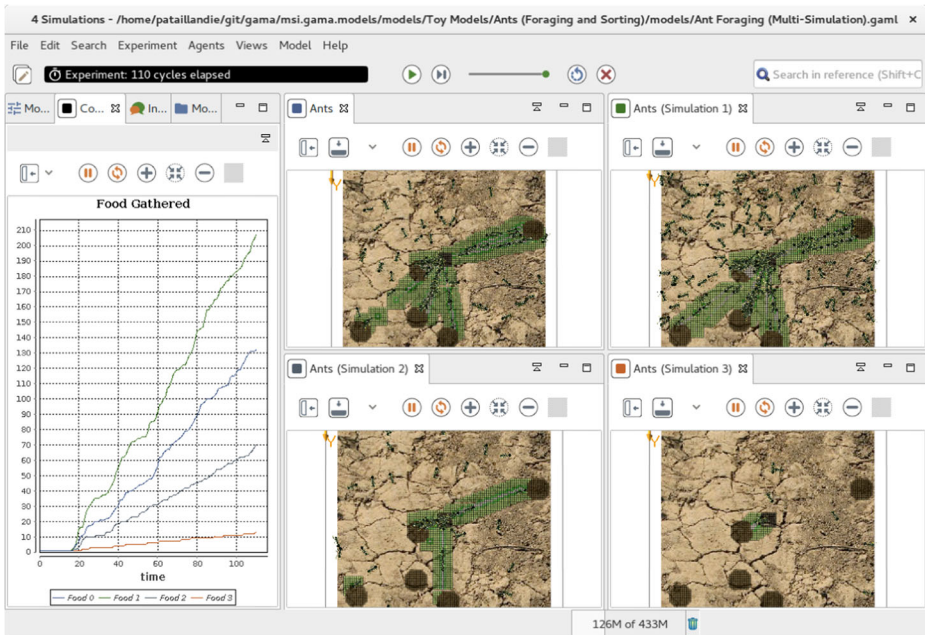
Fig. 5 Example of use of multi-simulation: 4 simulations concerning ant foraging are run in parallel with 4 different sets. The left chart shows in real time the results of the 4 simulations in terms of food gathered
