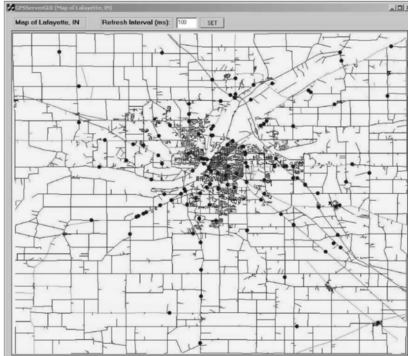
Figure 4. Server GUI.
