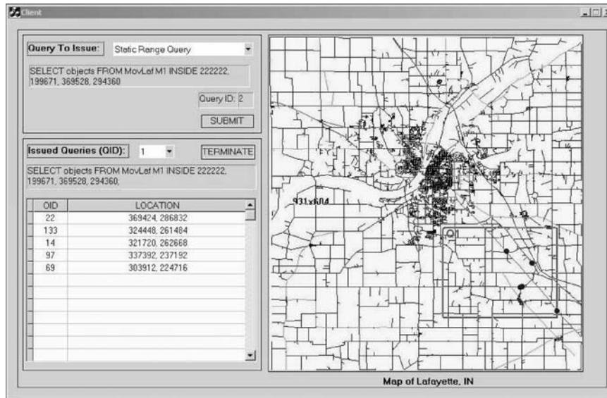
Figure 5. Client GUI.
