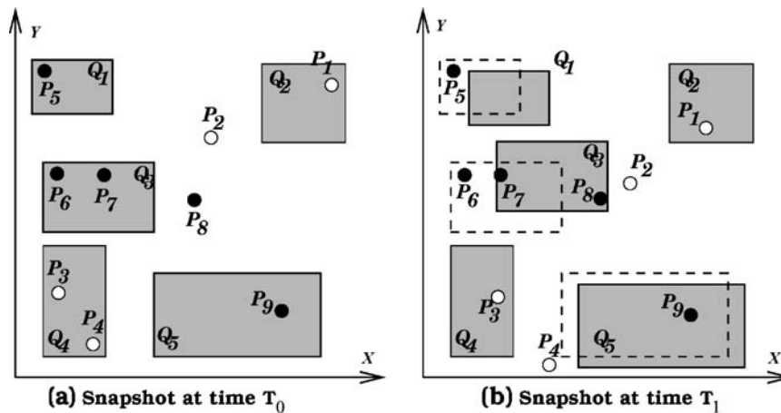
Figure 2. Incremental evaluation of range queries.
