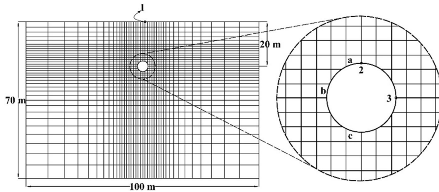
Fig. 3 A view of the meshed zone to analyze with FLAC software using the Finite-Difference Method (FDM)
