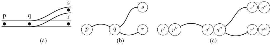
Fig. 16 a On the railway network, paths p - q - r and p - q - s exist, in both directions. b In a conventional undirected graph representation, there would also be a path r - q - s . c When the graph is extended to include two sides of each node, there is no longer a path r - q - s
