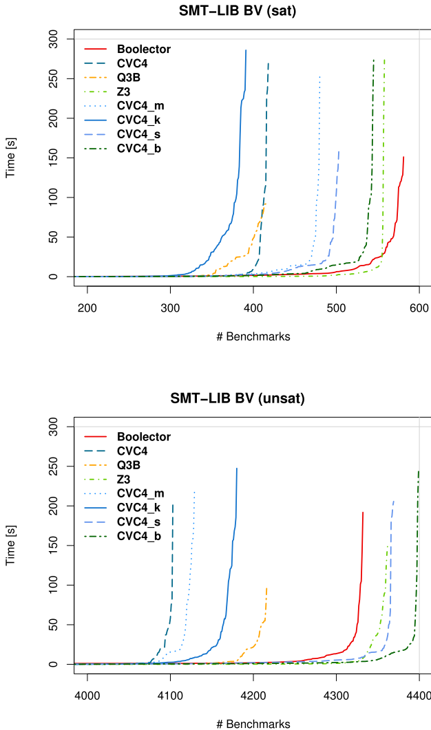
Fig. 5 (Un)satisfiable results on all BV benchmarks with a 300 second time limit
