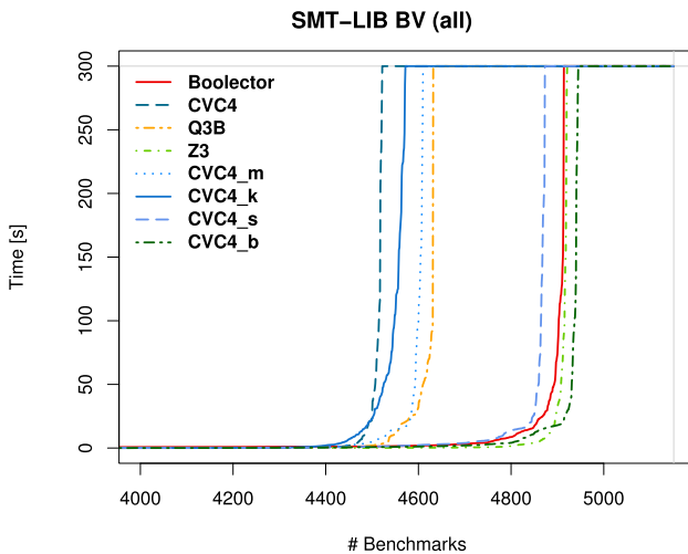
Fig. 4 Results on all BV benchmarks with a 300 second time limit
