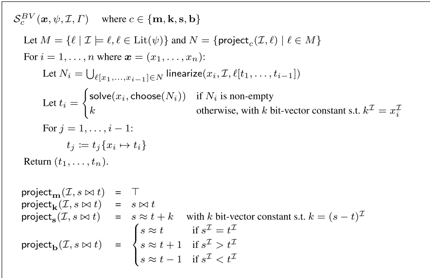
Fig. 3 Selection functions S_c^{BV} for binder-free bit-vector formulas. The procedure is parameterized by a configuration c , one of either m (model value), k (keep), s (slack), or b (boundary)
