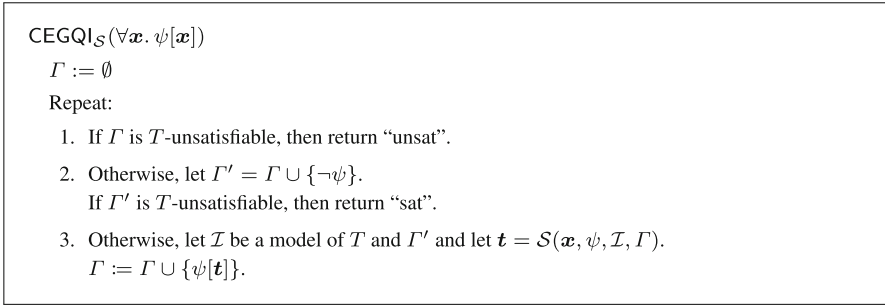
Fig. 2 A counterexample-guided quantifier instantiation procedure CEGQI S , parameterized by a selection function \mathcal{S} , for determining the T -satisfiability of \forall \mathbf{x}. \psi with \psi binder-free
