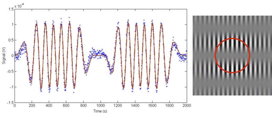
Fig. 2 The left panel shows the planet signal detected with the Planet Detection Testbed [47]. Each point is an item of data from the 2-s chop cycle and the whole trace shows the null signal obtained over a 360 degree effective rotation of the interferometer array. The line is a fit to the signal from a planet at a nominal angular radius of 6.35 \times 10^{-7} rad (or 132 mas) from the star. By comparison, the equivalent angular fringe distance from the short baseline is 4.7 \times 10^{-7} rad. Near the center and at the ends of the plot, the planet crosses the null fringe. The right panel shows the equivalent sensitivity map of the interferometer array. Array rotation causes the planet location to orbit (solid line) around the central null fringe (gray), and thus its signal is modulated both by the higher frequency fringes on the long baseline and by the chopping. Note that this demonstration was realized at room temperature with high flux levels. Technological developments are required to repeat this demonstration in cryogenic conditions with optical fluxes similar to those expected from astronomical sources (see Section 4.3)
