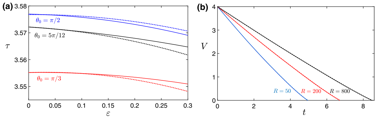
Fig. 7 a Droplet's lifetime as a function of the chemical pattern strength \varepsilon with average contact angle \pi/2 (blue), 5\pi/12 (black), and \pi/3 (red). The two modes of evaporation are also shown with a fixed centre position depicted with solid lines while the dot curves represent droplets which are free to translate along the substrate. b Volume time evolution for different cases of the parameter R , namely R = 50, 200 and 800 for the blue, red and black curves, respectively. The solid/dashed lines correspond to droplets which are fixed/move freely. In all cases, the pattern parameters are \theta_0 = \pi/3 and \varepsilon = 0.3 . (Color figure online)
