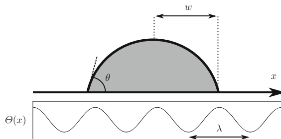
Fig. 1 A two-dimensional droplet resting on a flat solid surface with a smooth chemical pattern that is quantified in terms of the equilibrium contact angle \Theta(x) . The wavelength of the pattern is \lambda and the droplet’s footprint is denoted by w . The circular shape of the droplet is quantified in terms of the contact angle \theta , which is the same on both contact points
