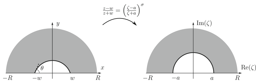
Fig. 2 Diagram showing how a circular segment with angle \theta and width w is mapped to the upper semi-circle with radius a = w/\sigma using (10), where \sigma = 2(1 - \theta/\pi) . The grey shaded region in the left diagram is a depiction of \Omega , and in the right diagram, it depicts the transformed domain
