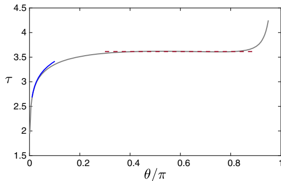
Fig. 5 The lifetime of a droplet evaporating, from an initial volume of V_0 = 2 on a smooth surface with no patterning depicted (i.e. \varepsilon = 0 ) as a function of the contact angle. Blue solid line and red dashed line represent the two special cases of extremely hydrophilic conditions, Eq. (28), and neutral wetting conditions, Eq. (30), respectively. (Color figure online)
