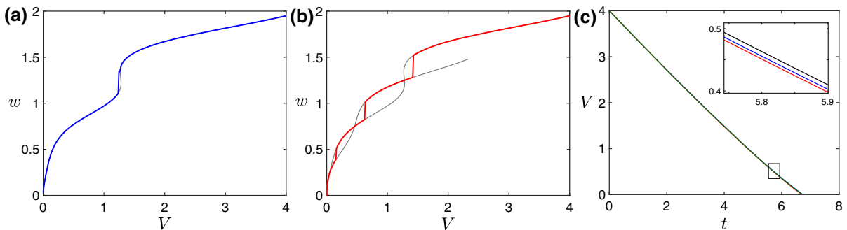
Fig. 6 a Droplet’s width as function of the volume when the droplet remains fixed at the same location without lateral shift. The underlying grey line denotes the bifurcation diagram of equilibrium solutions from Sect. 4. b Droplet’s width as function of the volume when the droplet is allowed to shift at each pitchfork bifurcation. The underlying grey lines show the corresponding bifurcation diagrams. In both a and b the strength of the chemical pattern is \varepsilon = 0.2 . c Time evolution of the droplet’s volume. The inset shows a magnified plot of the region marked with a rectangle, where the blue and red lines correspond to the cases of (a) and (b), respectively, and the black line corresponds to a homogeneous surface ( \varepsilon = 0 ). In all cases the average contact angle is \theta_0 = \pi/3 . (Color figure online)
