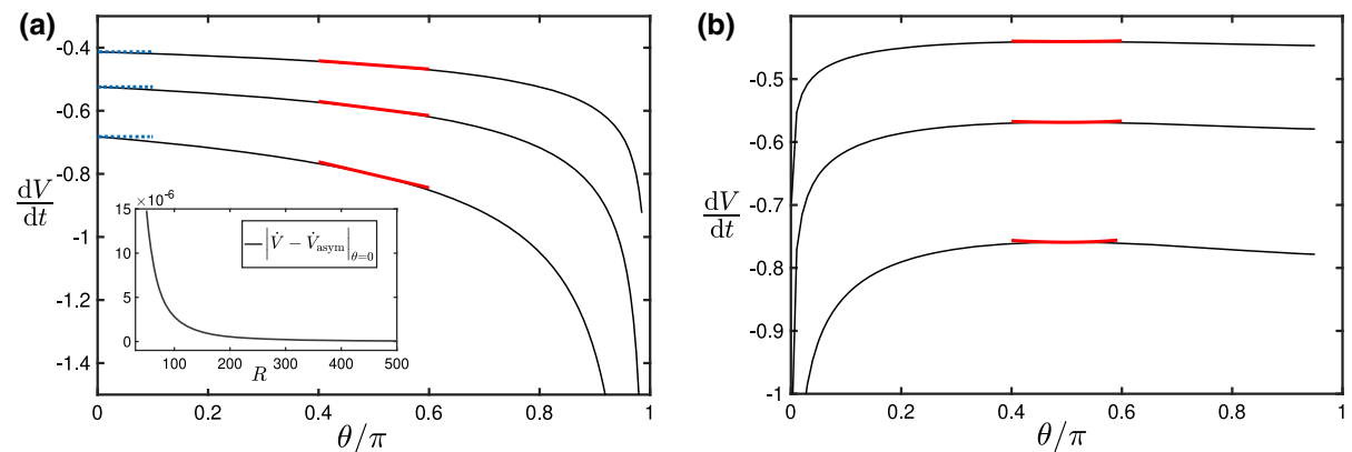
Fig. 3 Evaporation rates given by Eq. (14) with w = 1 (a) and V = 1 (b). The three curves correspond (from bottom to top) to R = 50, 200, 1000 , respectively. Red lines in panels a and b correspond to the evaporation rates given by Eq. (18) (neutral wetting), and blue dashed lines in panel a are plots of Eq. (22) (complete wetting limit). The inset panel in a shows the difference between the numerical results from Eq. (14) and the asymptotic result (22) as a function of R . (Color figure online)
