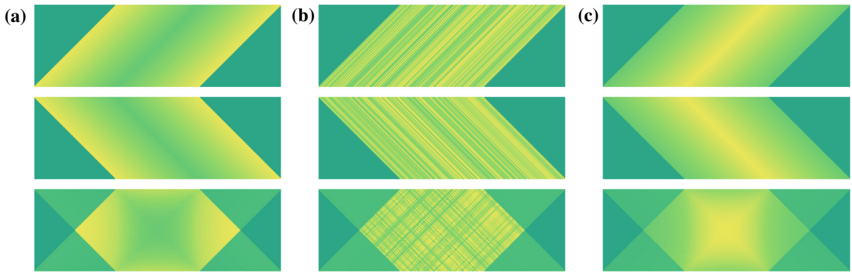
Fig. 8 First gradient shear energy model – contour plots of rotations \vartheta_{1,ij} , \vartheta_{2,ij} and \vartheta_{1,ij} + \vartheta_{2,ij} (yellow contours represent greater values than green contours), for the imposed displacements: a u_1 = u_2 = 0.65 < u_c , b u_1 = u_2 = u_c = \sqrt{3} - 1 , c u_1 = u_2 = 0.8 > u_c
