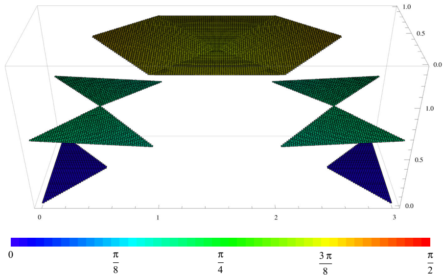
Fig. 13 First gradient quartic energy model – relative rotation, \vartheta_{1,ij} + \vartheta_{2,ij} , for free end displacement u_1 = u_2 = 0.8
