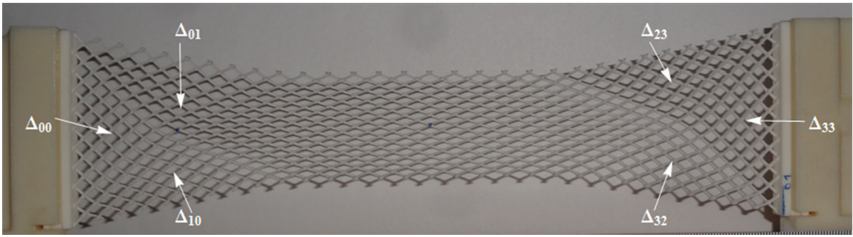
Fig. 4 Photograph of 3D-printed pantographic specimen under bias extension test. The regions \Delta_{00} , \Delta_{01} , \Delta_{10} , \Delta_{23} , \Delta_{32} and \Delta_{33} are highlighted (see also Fig. 2a). It is clear that the regions \Delta_{00} and \Delta_{33} are undeformed
