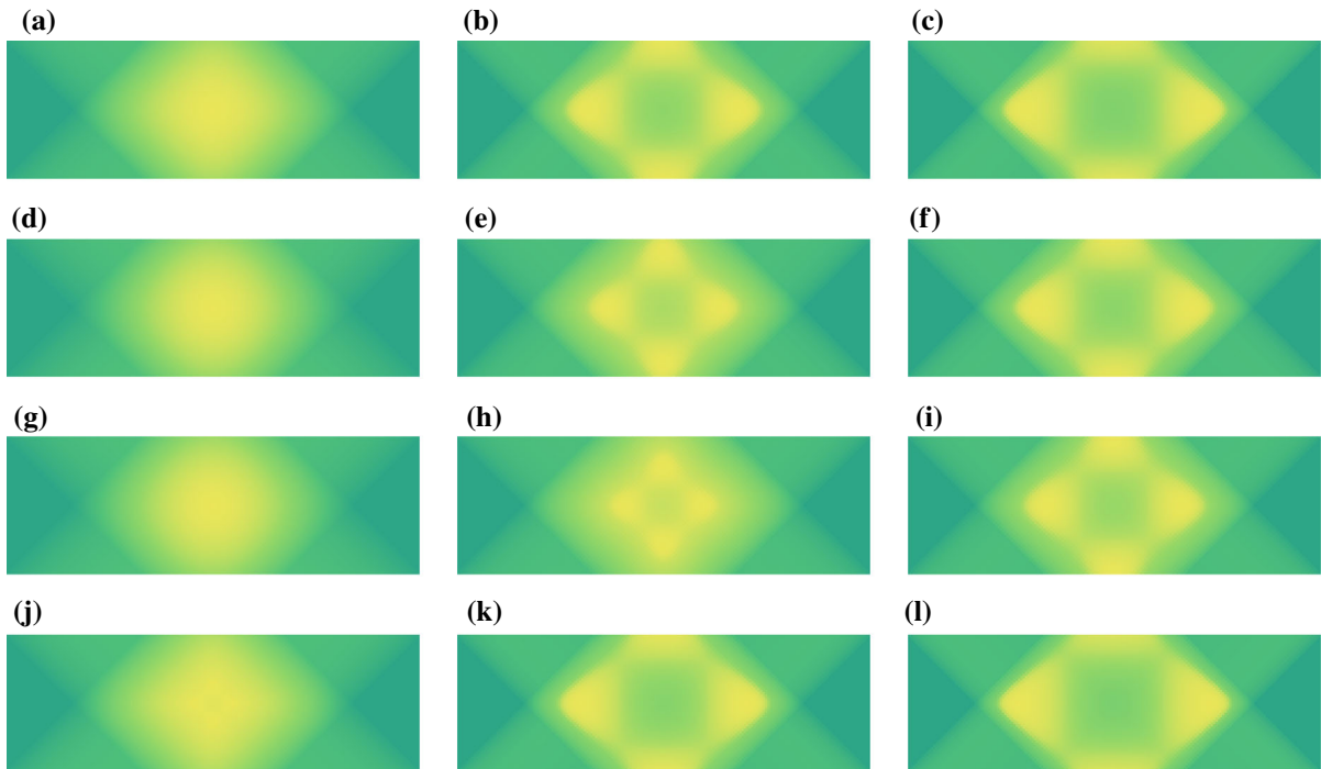
Fig. 30 Comparison of distribution of \vartheta_{ij} = \vartheta_{1ij} + \vartheta_{2ij} for displacement u_1 = u_2 = 0.6 and \beta = 1 for several increasing values of \alpha = 5, 25 and \alpha = 50 for the four first and second gradient energy models – QQ model: a \alpha = 5 , b \alpha = 25 , c \alpha = 50 ; SS model: d \alpha = 5 , e \alpha = 25 , f \alpha = 50 ; SQ model: g \alpha = 5 , h \alpha = 25 , i \alpha = 50 ; QS model: j \alpha = 5 , k \alpha = 25 , l \alpha = 50
