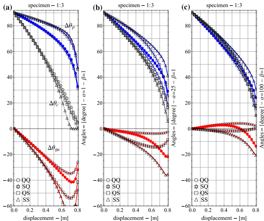
Fig. 31 Comparison of indicator angles for several energy models: a second gradient–dominated range, b transition range, c first gradient–dominated range
