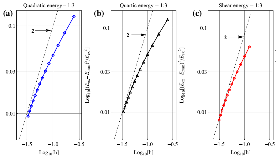
Fig. 6 Convergence analysis: square of relative energy error versus mesh size, h , for a quadratic, b quartic and c shear energy first gradient models
