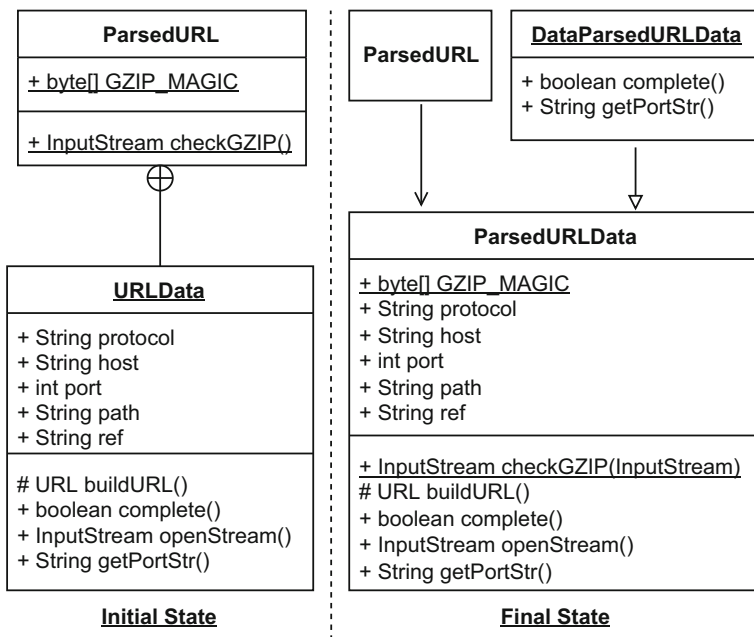
Fig. 3 Graphical representation of the Extract Superclass refactoring applied in revision e28370d2 in project BATIK
