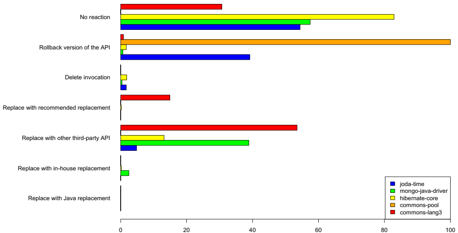
Fig. 7 Percentage breakdown of frequency of reaction patterns for the ‘joda-time’, ‘mongo-java-driver’, ‘hibernate-core’, ‘commons-pool’ and ‘commons-lang3’ APIs
