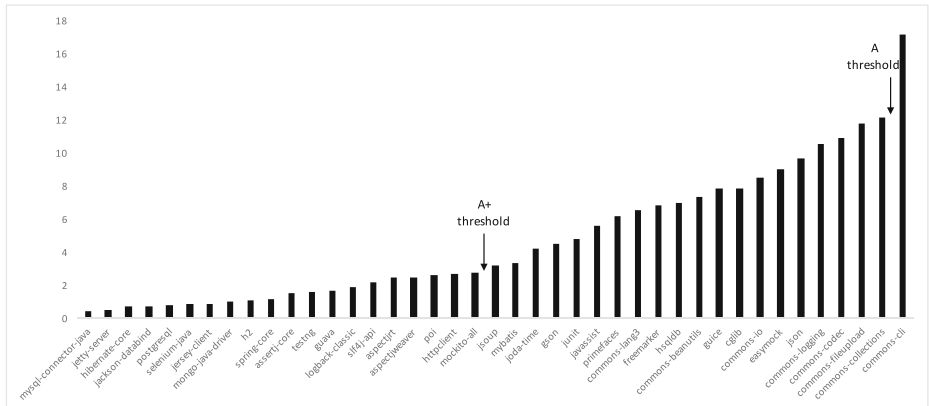
Fig. 8 Activeness of APIs, excluding inactive APIs
