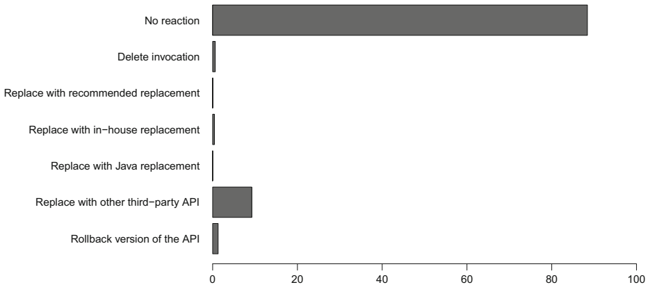
Fig. 3 Percentage distribution of reaction patterns
