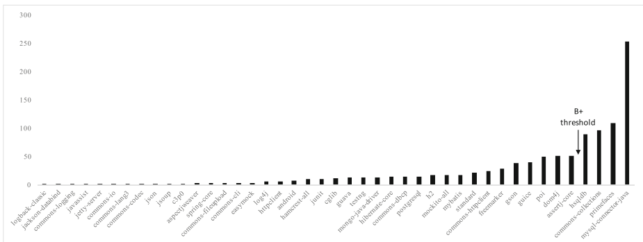
Fig. 11 Frequency of breaking features, excluding APIs that never directly introducing breaking changes
