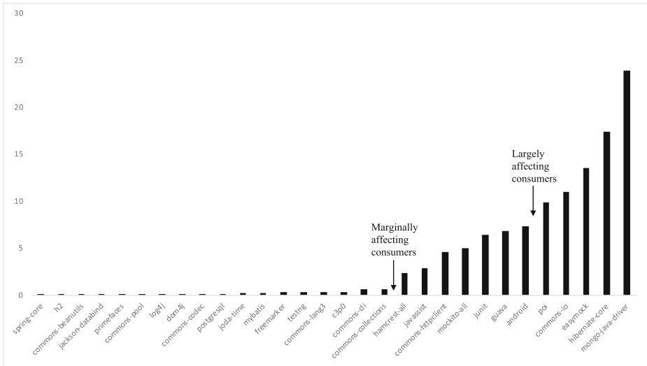
Fig. 5 Percentage of consumers affected per API
