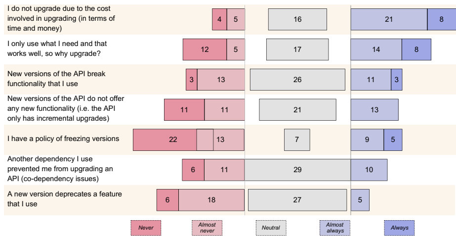
Fig. 2 Reasons behind not upgrading a dependency
