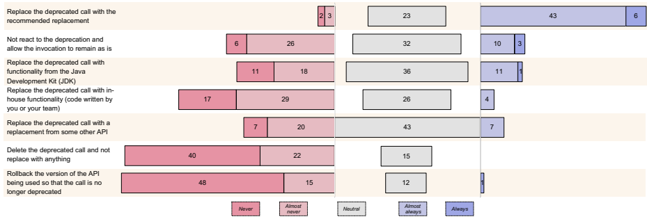
Fig. 4 API consumers’ preferred way to react to deprecation
