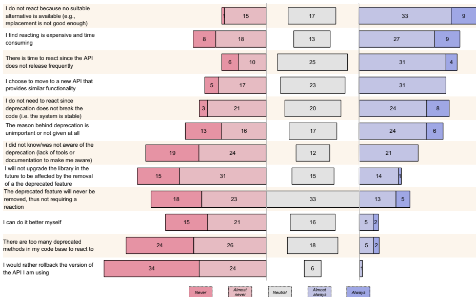
Fig. 12 API consumers reasons for not reacting to deprecation
