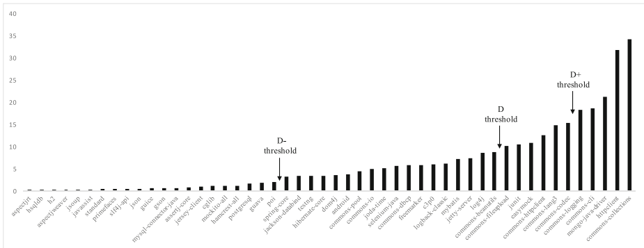
Fig. 10 Frequency of deprecating features, excluding APIs that do not deprecate at all
