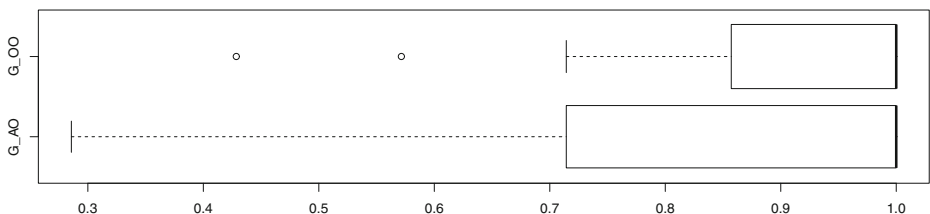
Fig. 6 Box plot of comprehension accuracy by group
