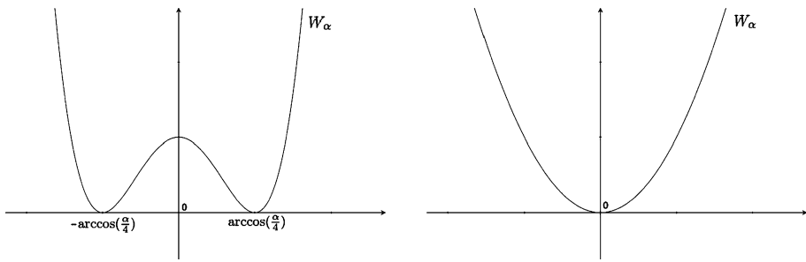
Fig. 2 The potential W_\alpha for 0 \leq \alpha < 4 (on the left) and for \alpha \geq 4 (on the right)
