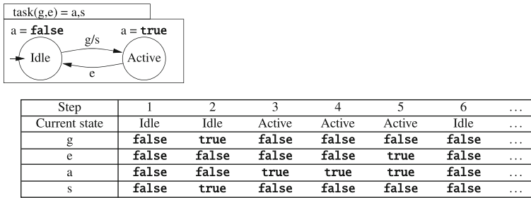
Fig. 3 Basic task control
