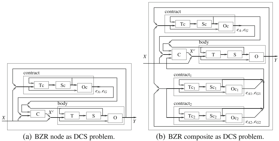
Fig. 14 BZR and DCS problem
