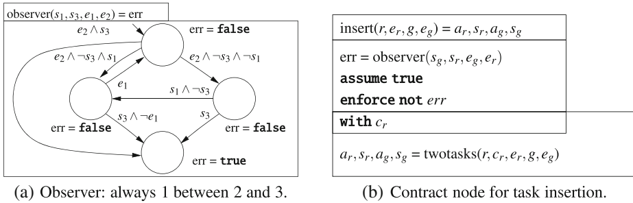
Fig. 9 Observer and contract node
