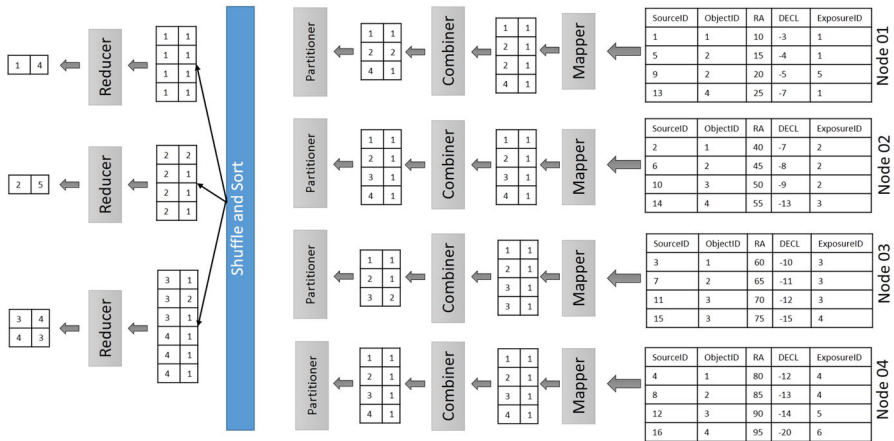
Fig. 1 Illustration of sample query processing using MapReduce
