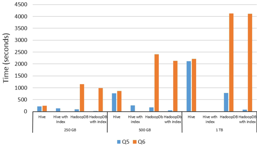
Fig. 8 GROUP BY tasks: Hive versus HadoopDB
