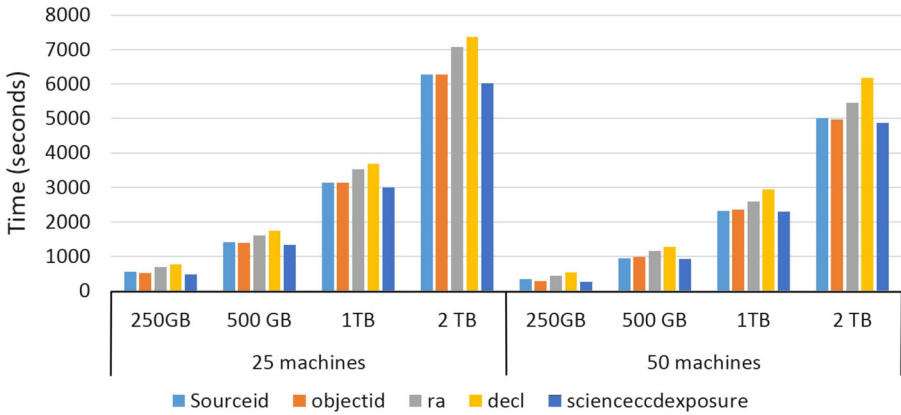
Fig. 3 Hive: data indexing
