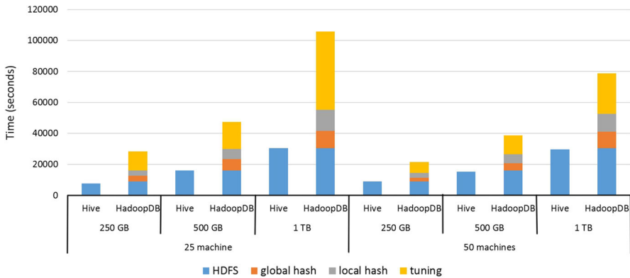
Fig. 2 Data loading: Hive versus HadoopDB
