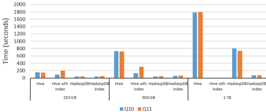
Fig. 11 ORDER BY tasks
