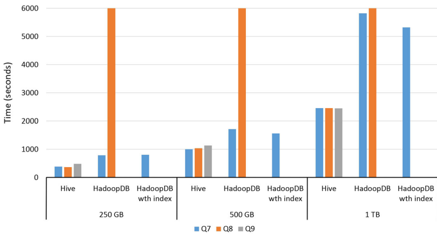
Fig. 10 JOIN tasks
