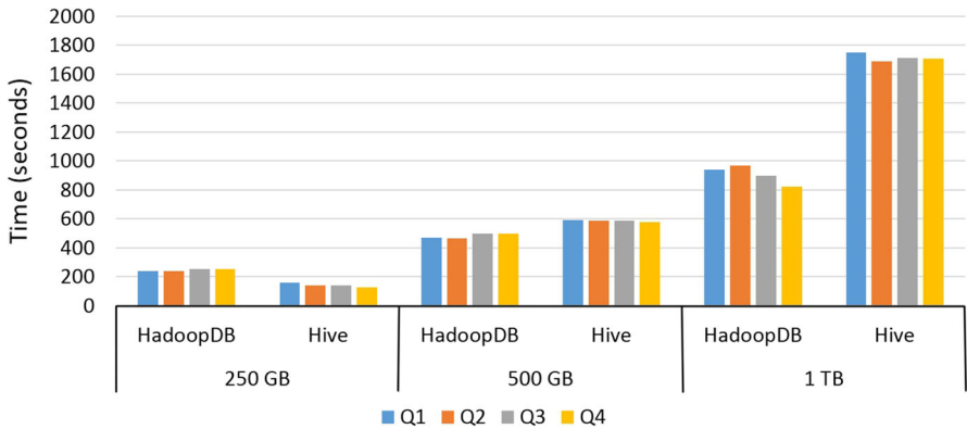
Fig. 6 SELECTION tasks without index
