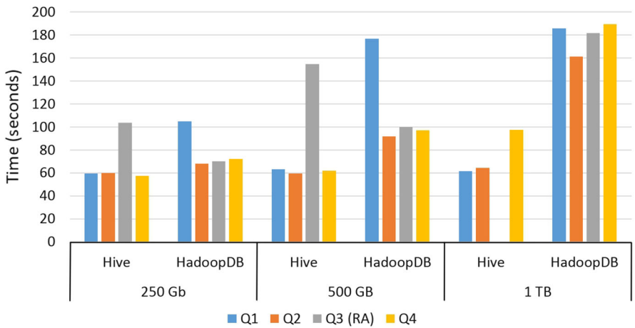
Fig. 7 SELECTION tasks with index
