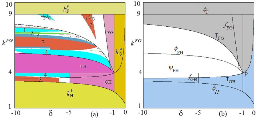
Fig. 2 Two dimensional bifurcation diagram in the parameter plane (\delta, k^{FG}) for C = 3, k^{FH} = 1 and \epsilon = 0.2 . In a the fixed points and the 2-cycles have regions in yellow and pink, respectively, with different tonalities, depending on the symbolic sequence. Red color corresponds to a 3-cycle, azure color to a 4-cycle, green color to a 5-cycle, while white regions correspond to chaotic intervals. b The bifurcation curves are shown, and in the gray (resp. light blue) region the interval I_{FG} (resp. I_{GH} ) is absorbing, in the white region the interval J is related to three branches of map T
