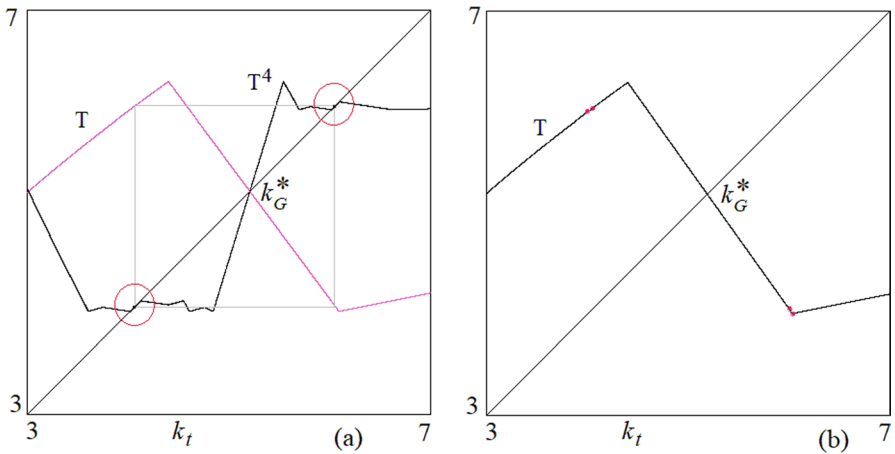
Fig. 5 k^{FG} = 4.4 , and the parameters as in Fig. 2. a \delta = -1.344995 , on the diagonal the circles are evidencing segments filled with 4-cycles; b \delta = -1.4 , a 4-cycle is the attracting set, evidenced by the red points
