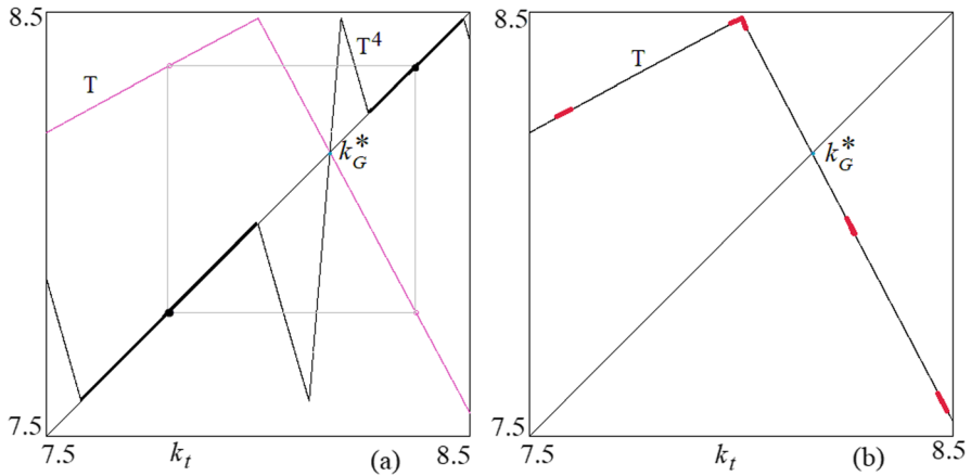
Fig. 4 k^{FG} = 8 , and the parameters as in Fig. 2. In a \delta = -1.860758 , on the diagonal are evidenced segments filled with 4-cycles; b \delta = -1.9 there are four chaotic intervals evidenced in red
