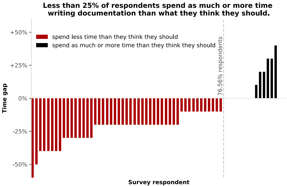
Figure 4. The gap between how much surveyed OSS library developers usually spend on documentation versus they time they think they should spend on documentation. Each vertical bar is a single respondent from a survey of developers at a scientific computing conference. Negative values represent respondents that believe they should spend more time on documentation, codified as “Documentation Guilt.” Figure created from data by Holdgraf and Varoquaux (2017).
