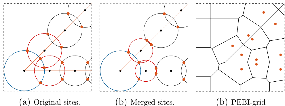
Fig. 13 Merging two conflict sites in a pinch-out. The orange lines are two intersecting fractures and red points the fracture sites
