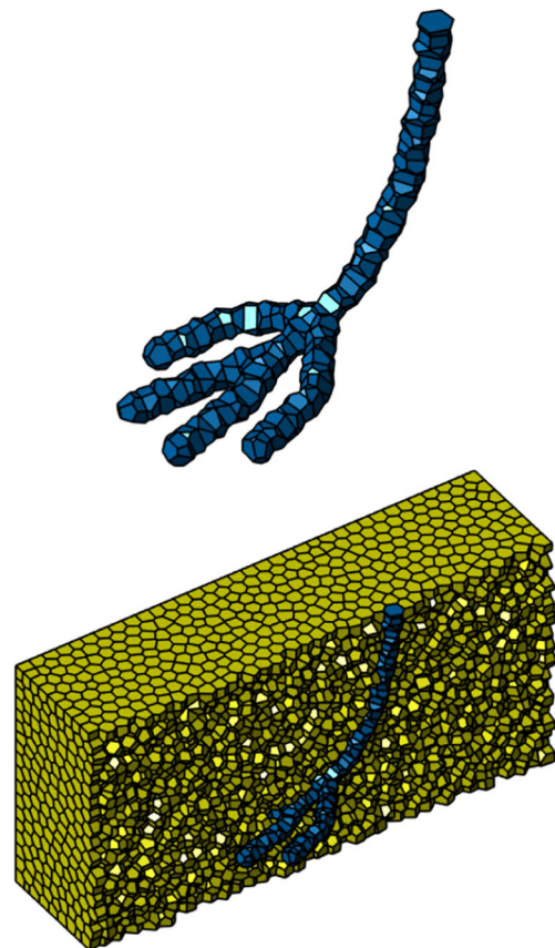
Fig. 23 A 3D grid with polyhedral Voronoi cells conforming to a well path
