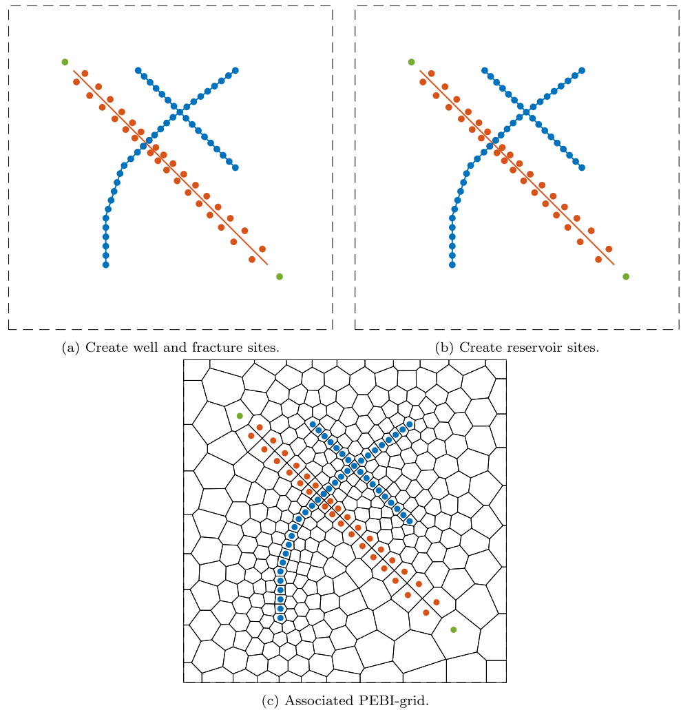
Fig. 18 Illustration of the overall algorithm used to generate grids with control-point alignment to two blue curves and boundary alignment to a red line. First, we generate well sites along the blue curves (blue dots), fracture sites (red dots) on opposite sides of the red lines and tip sites (green dots). Next, we distribute reservoir sites throughout the whole domain with a refinement towards the two well paths to generate a finer grid in the near-well region. In the last step, we first compute a Delaunay triangulation of the sites and then construct the corresponding clipped Voronoi diagram
