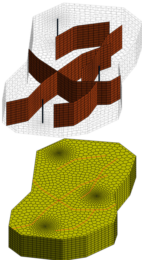
Fig. 22 A 2.5D grid of a fractured reservoir. The fracture faces and well cells in red and blue, respectively
