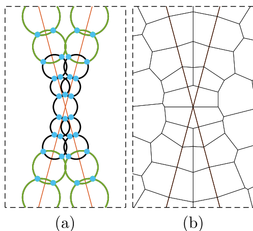
Fig. 15 An alternative to the merging procedure in Fig. 14. a Here two new 1D cells have been inserted for each fracture. The green circles are equal to those seen in Fig. 14a. The refinement towards the fracture intersection is enough to avoid the problems of non-intersection circles. If the intersection had been sharper a larger refinement would have been needed. b An associated grid
