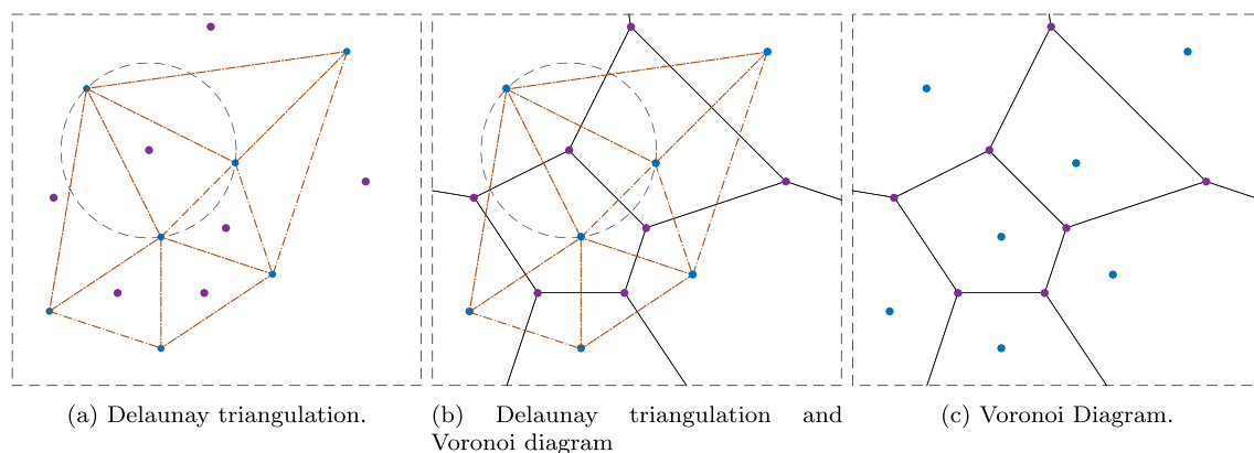
Fig. 1 Construction of a Voronoi grid from a point set by use of Delaunay triangulation. We start by specifying a set of generating points (blue dots), and then compute the corresponding Delaunay triangulation, defined so that no generating point falls inside the circumcircle of the triangles in the triangulation. The circumcenter (purple dots) of each triangle lies at the point where the three perpendicular bisectors of
