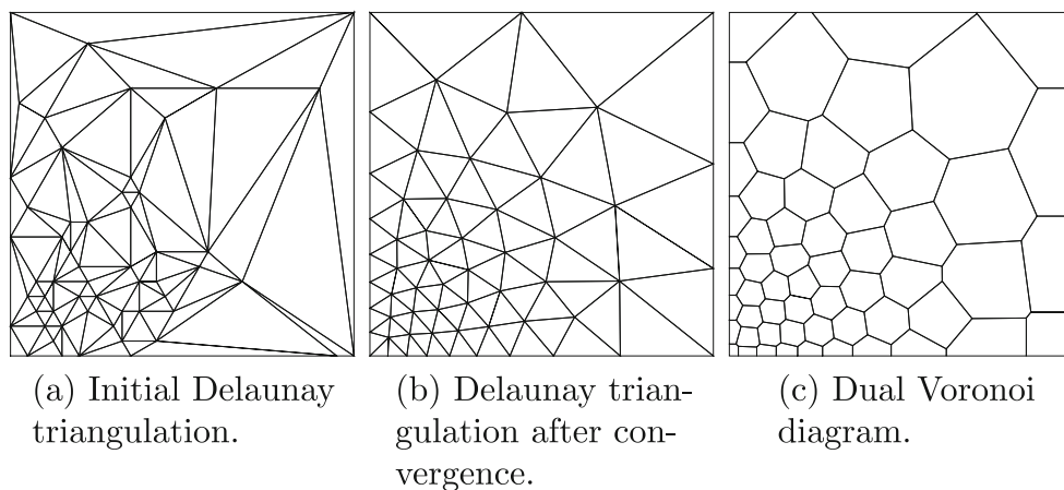
Fig. 26 Optimization of a triangulation using the force-based algorithm. The size of the elements is proportional to the distance from the origin squared h(x, y) \sim x^2 + y^2
