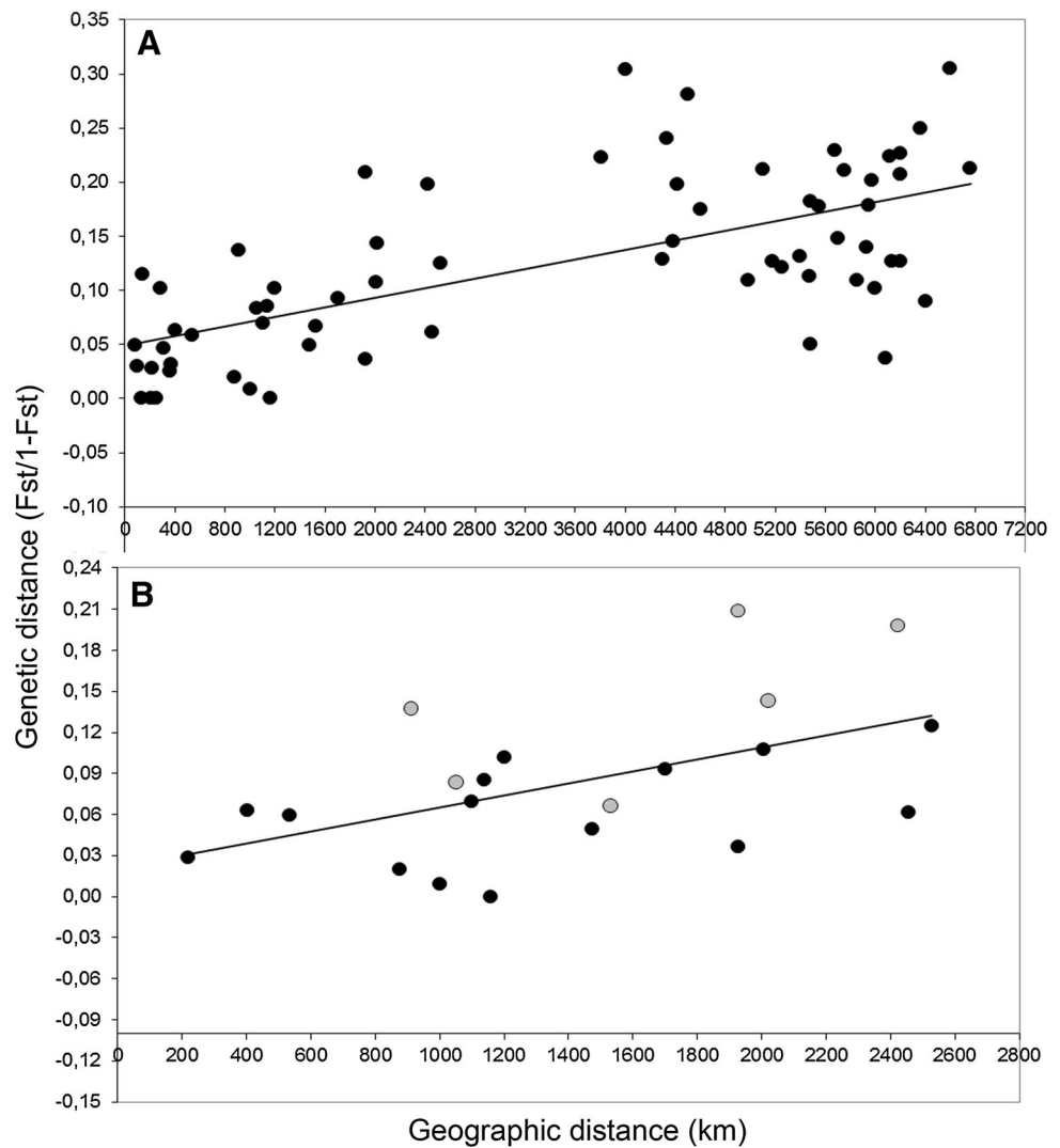
Fig. 2 Isolation by distance across jaguar populations. Pairwise genetic differentiation as F_{ST}/(1 - F_{ST}) at a multi-regional scale including Mexico ( n = 15 populations) and b regional scale; Brazil ( n = 9 populations). In grey , genetic comparisons involving CAPV, the easternmost Brazilian sampling site
