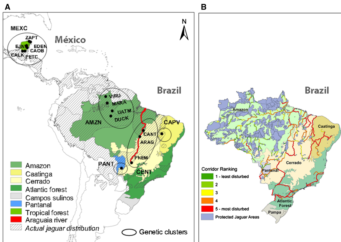
Fig. 1 a Map of the actual jaguar’s geographic range ( Panthera onca ), sampling sites (black points), genetic clusters and principal ecosystems in Brazil and Mexico (see details and codes in Table 1). The map is based on information from the IUCN Red List of
