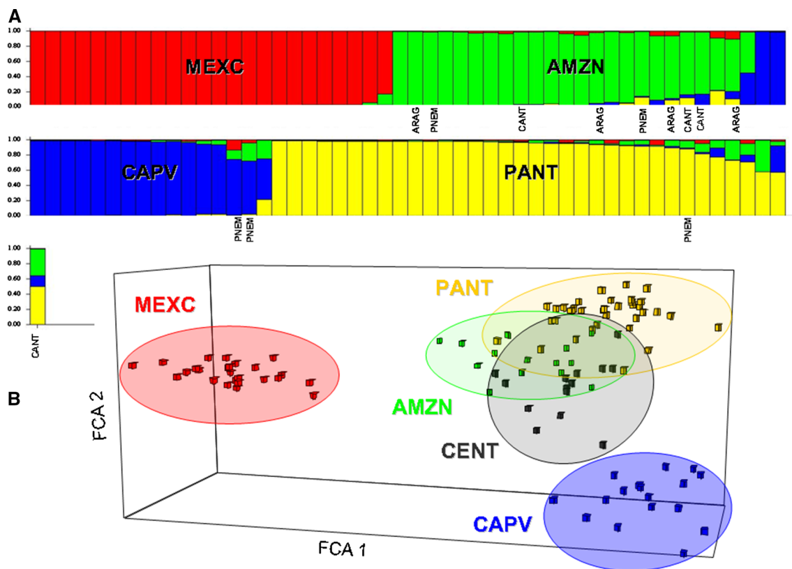
Fig. 3 a The genetic structure of the Brazilian populations identified by the STRUCTURE analysis assuming four genetic clusters ( K = 4 ; MEXC, AMZN, PANT and CAPV) in the overall population. Individuals are represented as bars partitioned into segments corresponding to their membership in genetic clusters indicated by the colors. Individuals from the Central areas (CENT: ARAG, PNEM, CANT) show from 50 to 100 % ancestry in AMZN, and the
