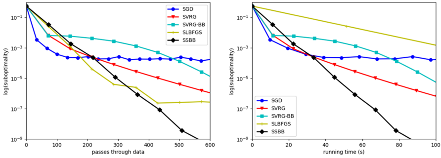
Fig. 2 l^2 -regularized logistic regression on w6a dataset from LIBSVM regularized with \lambda_2 = 10^{-4} . Left : number of passes through data. Right : running time
