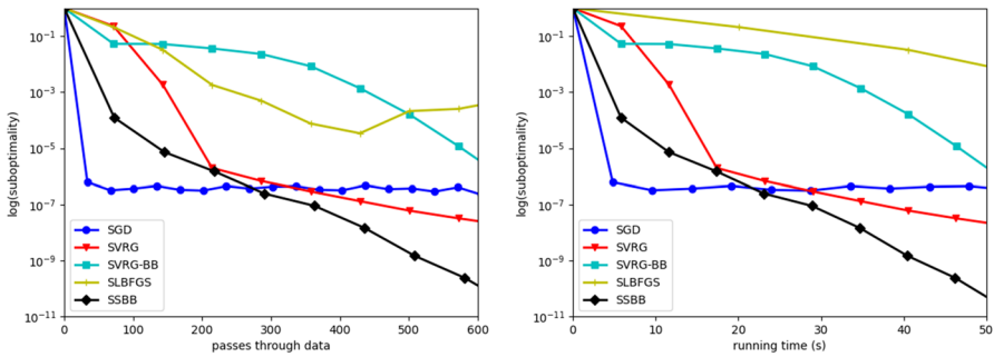
Fig. 3 l^2 -regularized squared hinge loss on a6a from LIBSVM regularized with \lambda_2 = 10^{-3} . Left : number of passes through data. Right : running time
