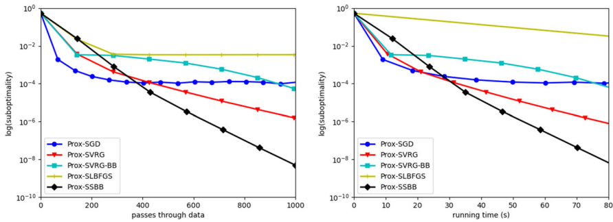
Fig. 4 Logistic regression with l^2 and l^1 regularizations on w6a dataset from LIBSVM regularized with \lambda_2 = 10^{-4} and \lambda_1 = 10^{-4} . Left : number of passes through data. Right : running time
