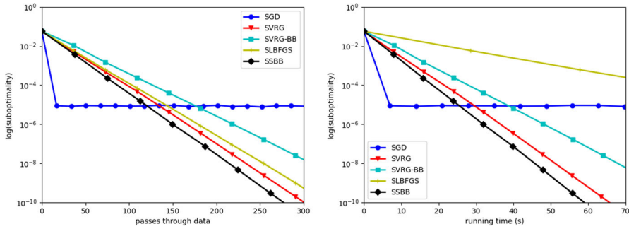
Fig. 1 Ridge regression on synthetic dataset regularized with \lambda_2 = 10^{-5} . Left : number of passes through data. Right : running time
