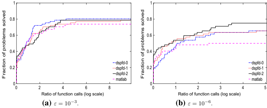
Fig. 1 Performance of three variants of Algorithm 2.1 and MATLAB patternsearch on bound-constrained problems
