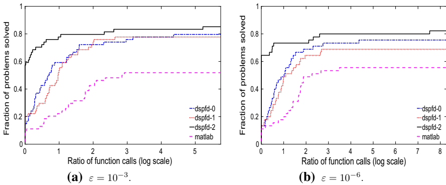
Fig. 5 Performance of three variants of Algorithm 2.1 and MATLAB patternsearch on problems with at least one linear equality constraint
