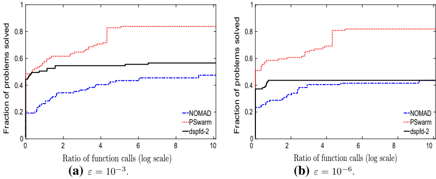
Fig. 7 Performance of Algorithm 2.1 (version 2) versus NOMAD and PSwarm on problems subject to general linear constraints. PSwarm was tested with a search step
