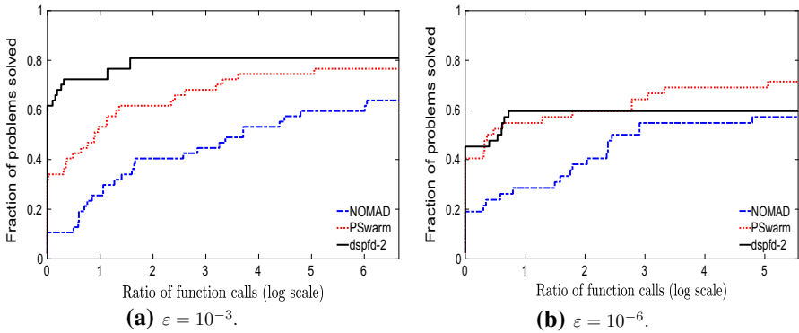
Fig. 8 Performance of Algorithm 2.1 (version 2) versus NOMAD and PSwarm on problems with at least one linear inequality constraint. PSwarm was tested with a search step
