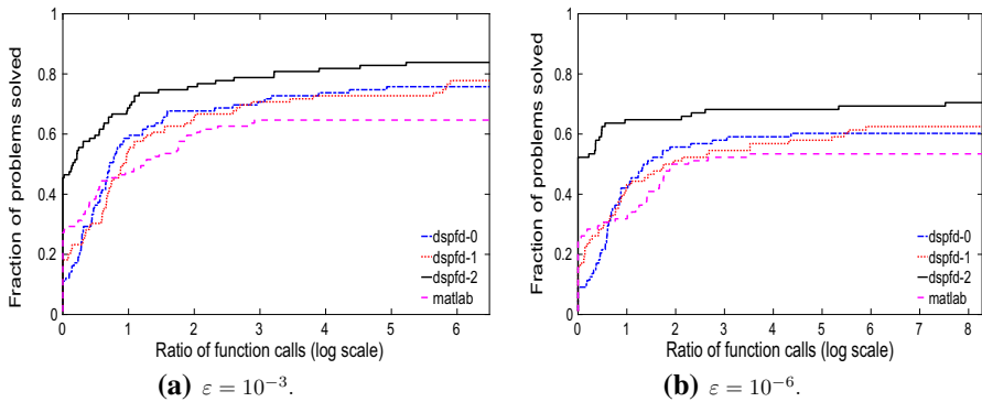
Fig. 3 Performance of three variants of Algorithm 2.1 and MATLAB patternsearch on problems subject to general linear constraints
