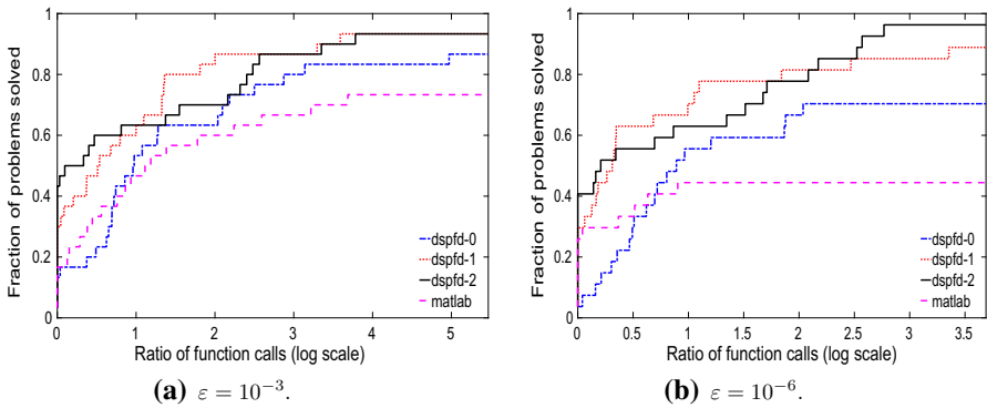
Fig. 2 Performance of three variants of Algorithm 2.1 and MATLAB patternsearch on larger bound-constrained problems
