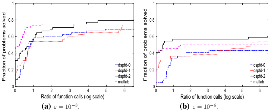
Fig. 4 Performance of three variants of Algorithm 2.1 and MATLAB patternsearch on problems with at least one linear inequality constraint
