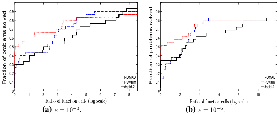
Fig. 6 Performance of Algorithm 2.1 (version 2) versus NOMAD and PSwarm on the largest tested bound-constrained problems. PSwarm was tested with a search step
