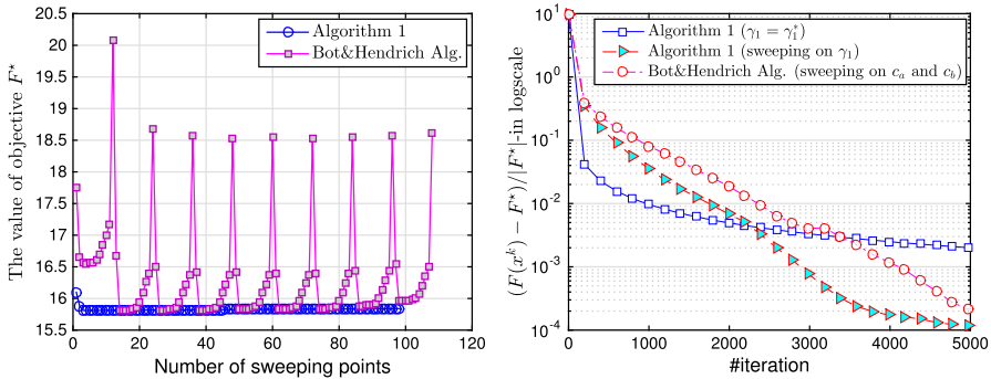
Fig. 3 Comparison of Algorithm 1 and Bot&Hendrich Alg. (left the objective values versus the number of sweeping points, right convergence of the relative objective residual)
