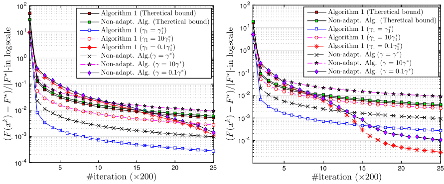
Fig. 2 The empirical performance versus the theoretical bounds of the 6 algorithmic variants ( left non-correlated data, right 50 %-correlated columns)
