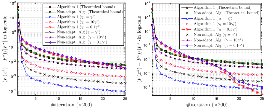
Fig. 1 The empirical performance versus the theoretical bounds of the 6 algorithmic variants ( left non-correlated data, right correlated data)
