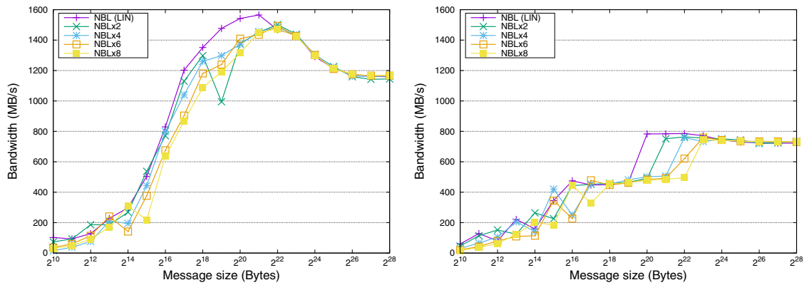
Fig. 5 Performance of the LIN algorithm for MPI_Iallgather in OpenMPI using 7 and 8 nodes/processes (left and right, respectively). The labels of type NBLxY indicate the pipelined variant MPI_Piallgather_fconc with numseg=Y segments
