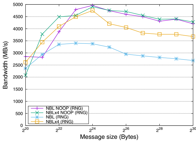
Fig. 4 Performance of the RNG algorithm in OpenMPI using 8 nodes/processes. The NBL NOOP suffix identifies the modified variant of MPI_Iallreduce without arithmetic operations; the labels of type NBL and NBLx4 respectively indicate the conventional variant MPI_Piallreduce_fconc and the pipelined alternative with numseg=4 segments
