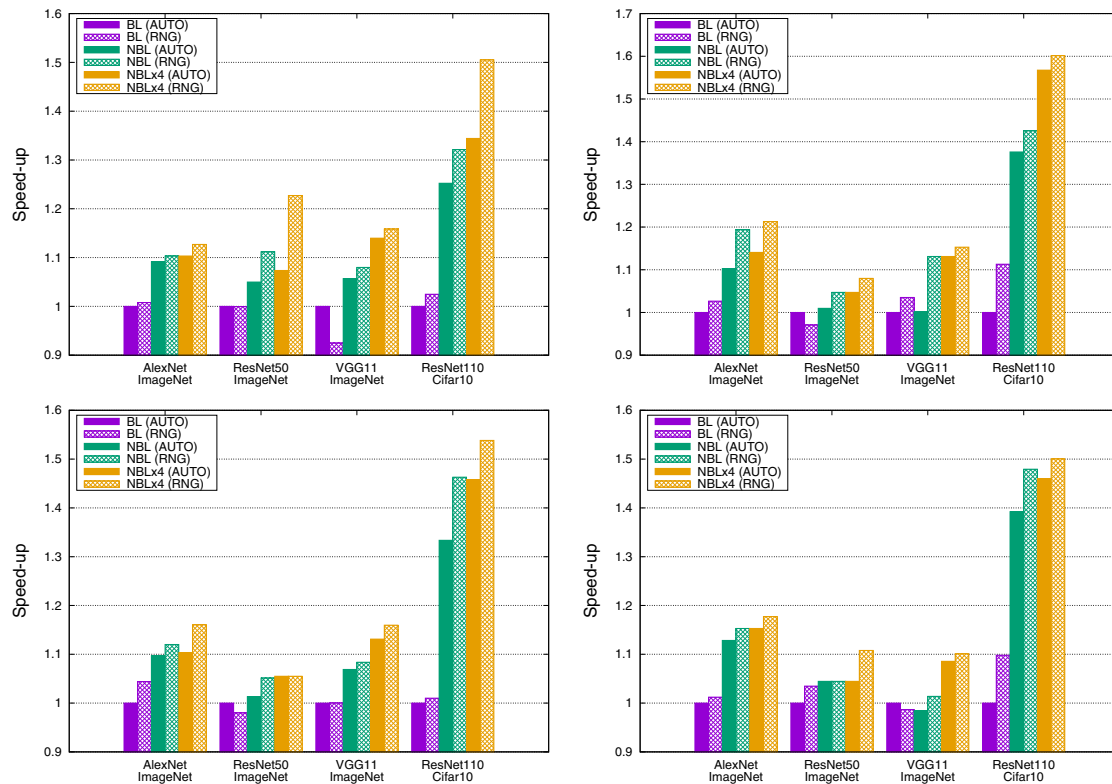
Fig. 9 Speed-up of TF+HVD when the blocking AUTO algorithm for MPI_Allreduce ( BL(AUTO) ) is replaced with either the blocking RNG algorithm ( BL(RNG) ), the non-blocking algorithms ( NBL(AUTO/RNG) ), or the pipelined variants of the latter
