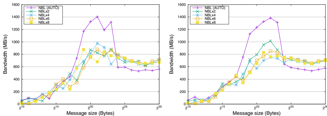
Fig. 7 Performance of the AUTO algorithm for MPI_Ireduce_scatter in OpenMPI using 7 and 8 nodes/processes (left and right, respectively). The labels of type NBLxY indicate the pipelined variant MPI_Pireduce_scatter_fconc with numseg=Y segments
