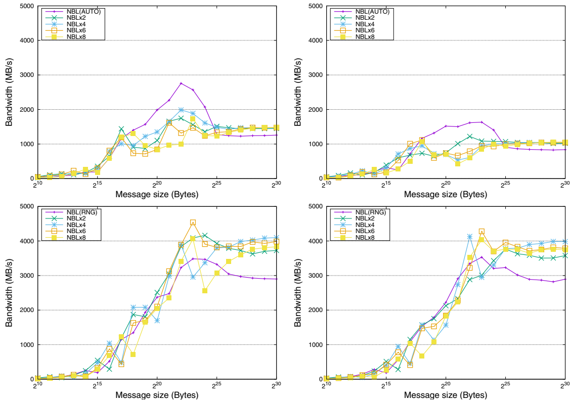
Fig. 3 Performance of the AUTO and RNG algorithms in OpenMPI (top and bottom, respectively) using 8 and 9 nodes/processes (left and right, respectively). The NBL(AUTO) and NBL(RNG) labels
