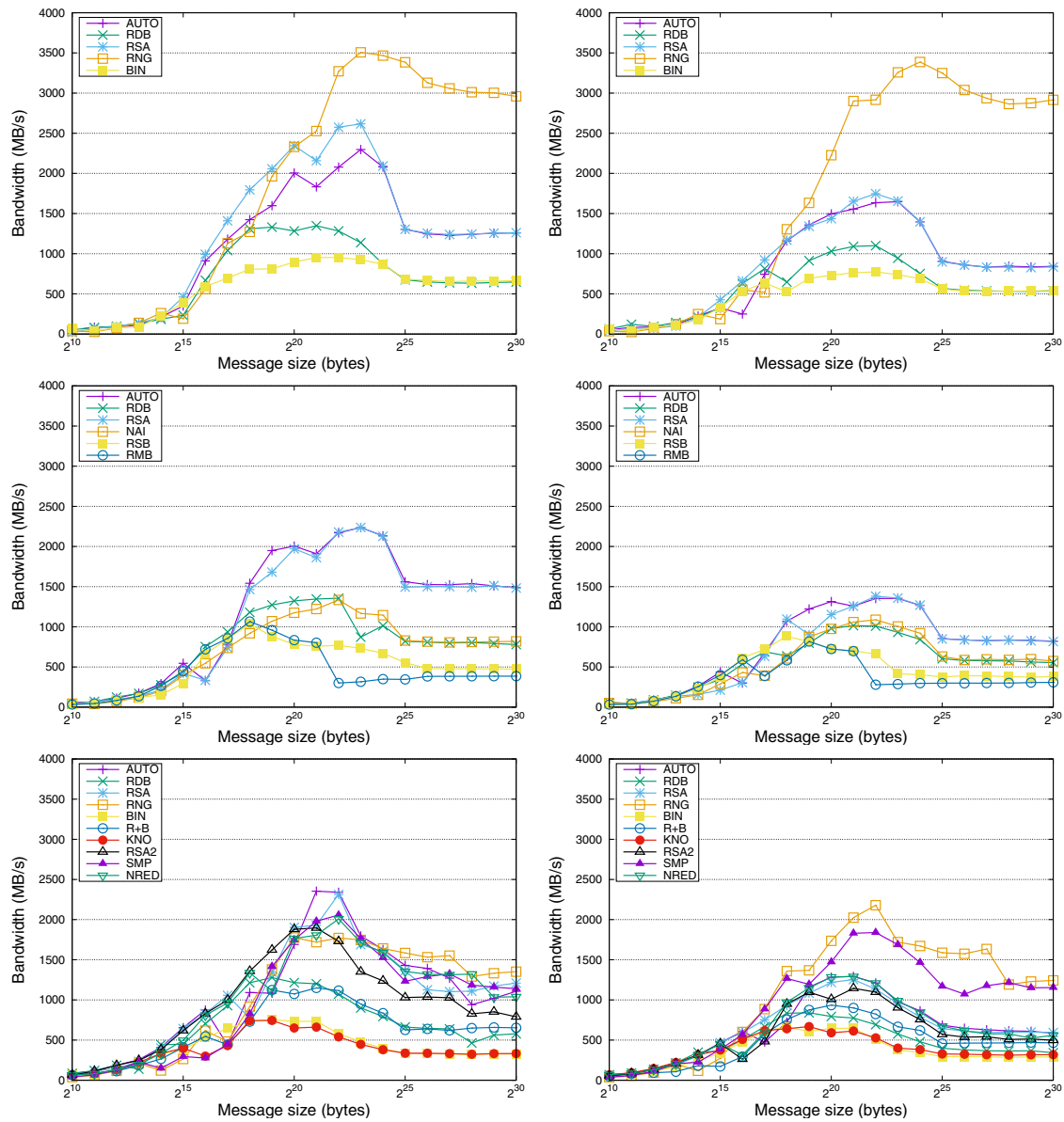
Fig. 1 Performance of the algorithms in OpenMPI, MPICH and Intel MPI for MPI_Iallreduce (top, middle and bottom, respectively) using 8 and 9 nodes/processes (left and right, respectively)
