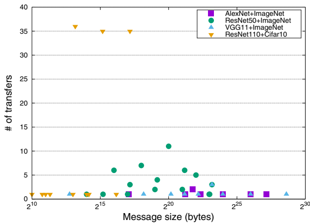
Fig. 8 Number of transfers clustered by message size for the DNN models+datasets
