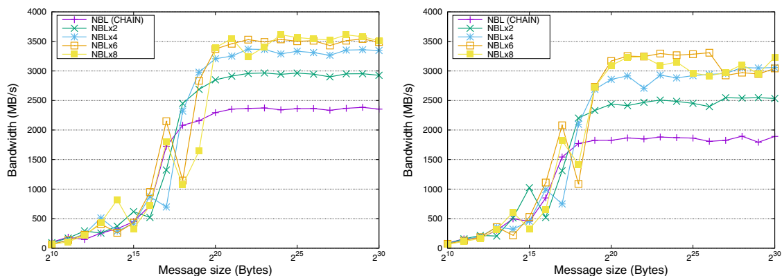
Fig. 6 Performance of the CHAIN algorithm for MPI_Ibcast in OpenMPI using 7 and 8 nodes/processes (left and right, respectively). The labels of type NBLxY indicate the pipelined variant MPI_Pibcast_fconc with numseg=Y segments
