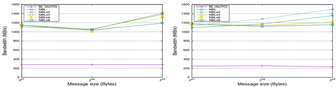
Fig. 14 Performance of the AUTO algorithm in OpenMPI (4.0) for large messages using 30 and 32 processes (left and right, respectively)
