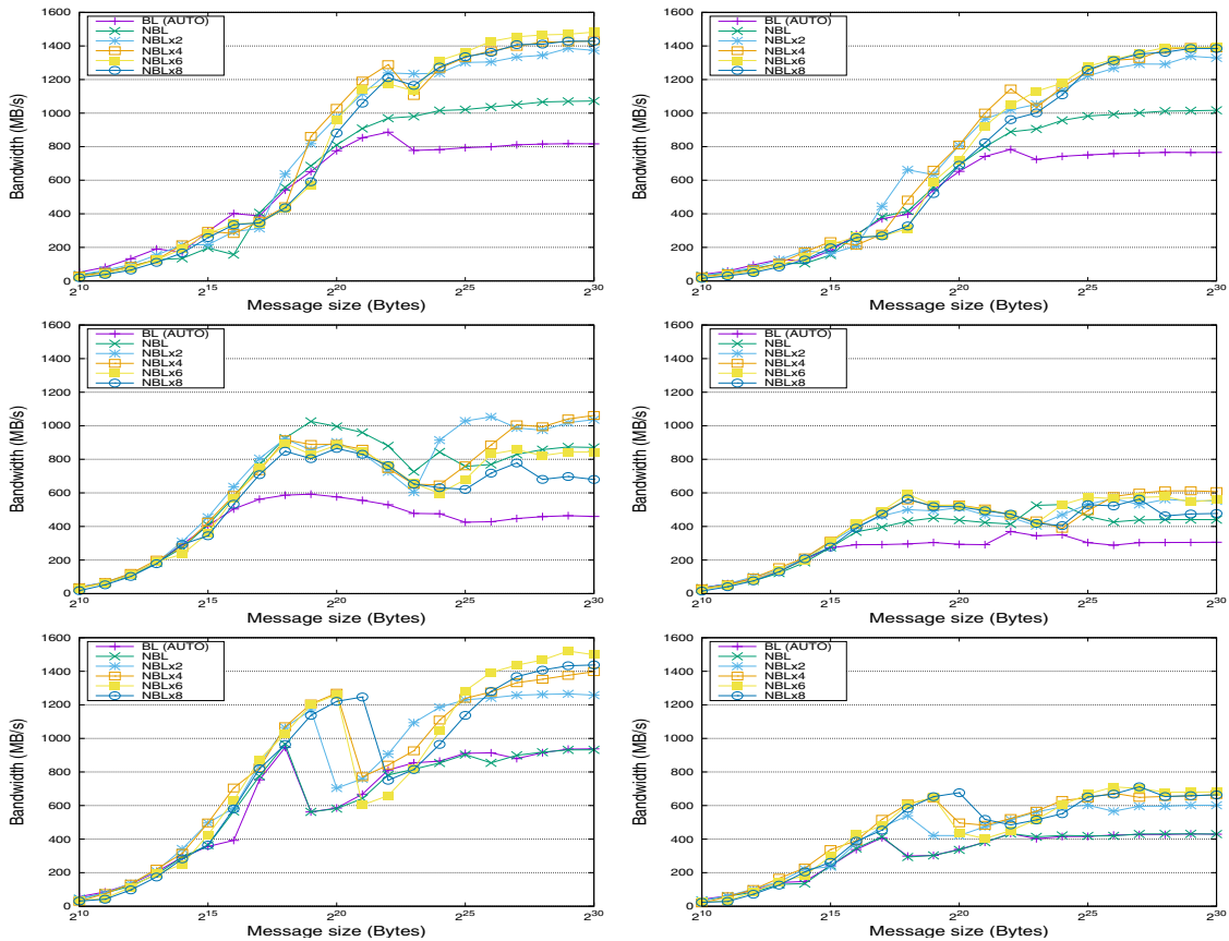
Fig. 13 Performance of the AUTO algorithm in OpenMPI 4.0 (top), and the AUTO and RNG algorithms in MPICH and Intel MPI (middle and bottom, respectively) using 8 and 15 nodes/processes (left and right, respectively)
