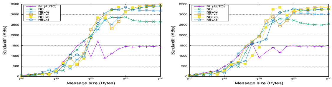
Fig. 12 Performance of the AUTO algorithm in OpenMPI (4.0) using 8 and 9 nodes/processes (left and right, respectively)
