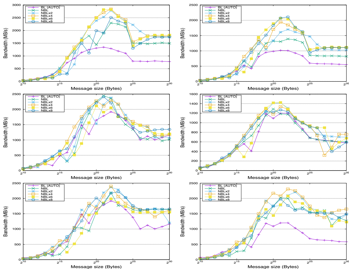
Fig. 11 Performance of the AUTO algorithm in MPICH (top), and the AUTO and RNG algorithms in Intel MPI (middle and bottom, respectively) using 8 and 9 nodes/processes (left and right, respectively)
