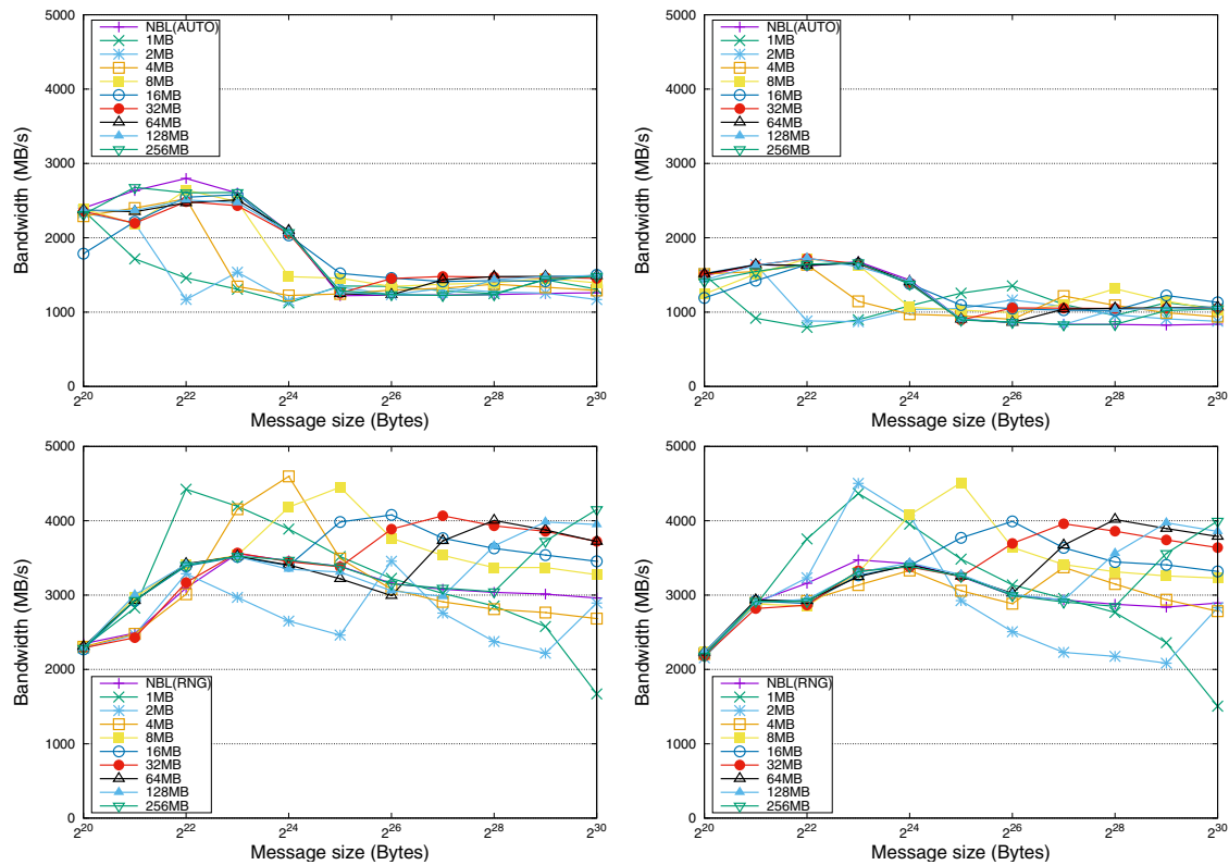
Fig. 2 Performance of the AUTO and RNG algorithms in OpenMPI (top and bottom, respectively) using 8 and 9 nodes/processes (left and right, respectively). The NBL(AUTO) and NBL(RNG) labels
