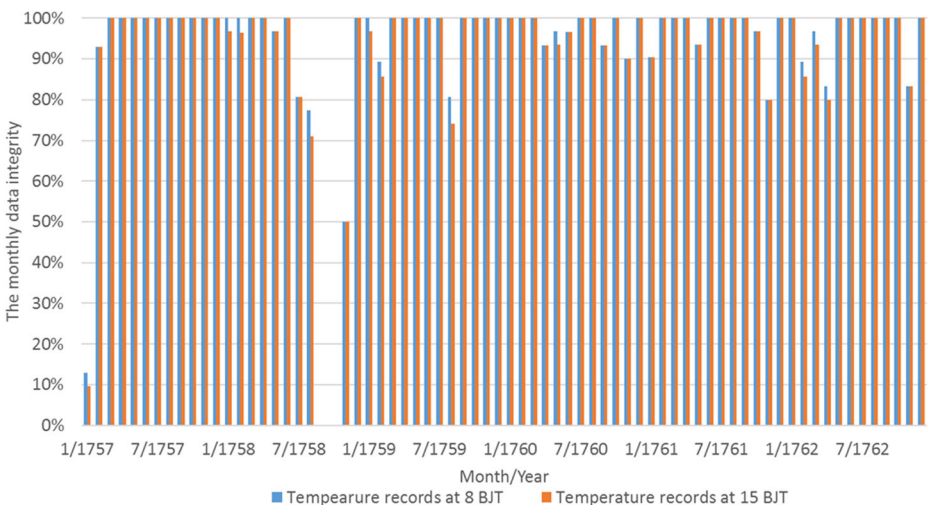
Fig. 2 The monthly ratio of the valid air temperature records at the Old North Church, Beijing
