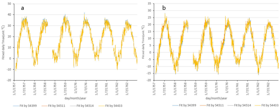
Fig. 12 The 1757–1762 daily T-max (a) and T-min (b) fit based on each of the four central urban stations
