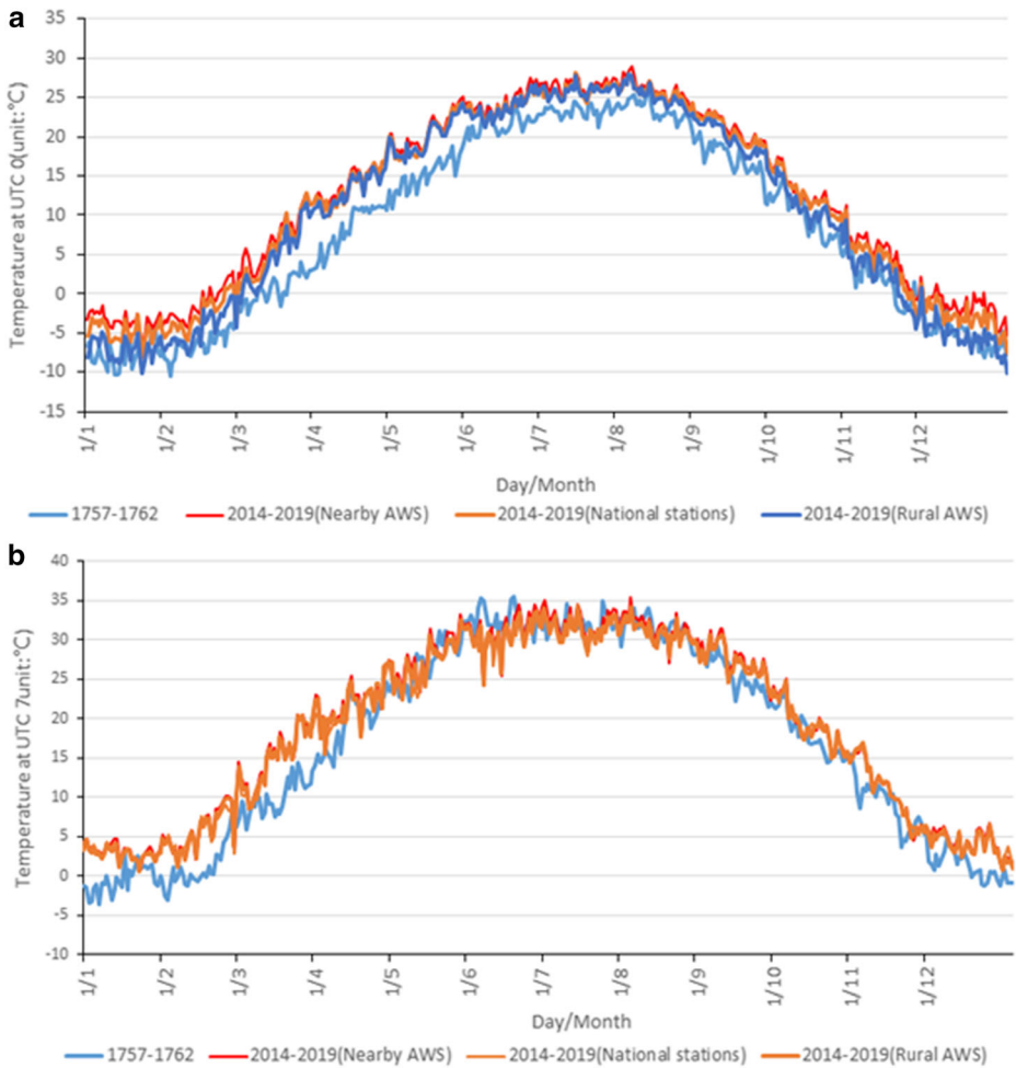
Fig. 3 Comparison of mean temperature at UTC 0 (a) and UTC 7 (b) for the different 6-year periods of 1757–1762, 1961–1967, and 2014–2019
