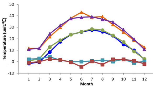
Fig. 7 The average of monthly maximum T-min and T-max during 2014–2019 and 1757–1762, and their differences between the two periods (unit °C)
