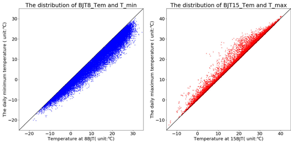
Fig. 4 The relationship between 8:00 BJT temperature and T-min (left), and 15:00 BJT temperature and T-max (right) at the four national stations in Beijing urban area (unit: °C)
