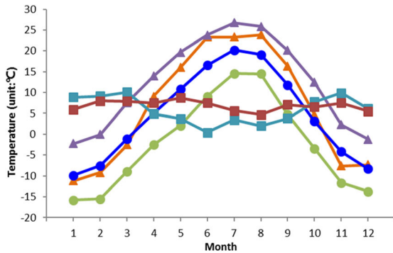
Fig. 6 The average of monthly minimum T-min and T-max during 2014–2019 and 1757–1762, and their differences between the two periods (modern-early years) (unit °C)
