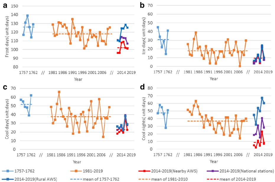
Fig. 10 The annual numbers of cold extreme events for periods of 1757–1762, 1981–2010, and 2014–2019 in Beijing (a FD0; b ID0; c, TX10p; d TN10p)
