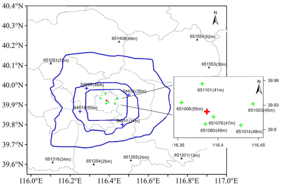
Fig. 1 The distribution of early observations (Old North Church) and the nearby national meteorological stations in Beijing (Red cross shows the location of Old North Church; Green cross shows the six nearest modern automatic meteorological stations (with observations of more than 10 years); Blue cross shows the four nearest modern national stations (with observations of more than 50 years) in different directions; Black triangle shows the eight rural automatic meteorological stations (with observations of more than 10 years); The numbers in brackets are altitudes of the stations in meter. The three hoops from inside to outside are the 4th Ring Road, 5th Ring Road, and 6th Ring Road, with the 4th Ring Road representing the central urban area of Beijing City
