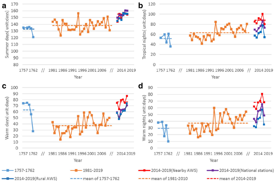
Fig. 9 The annual warm extreme events for periods of 1757–1762, 1981–2010, and 2014–2019 ( a SU25; b TR20; c TX90p; d TN90p)
