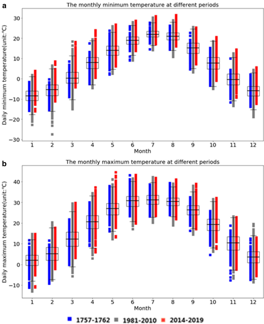
Fig. 8 The monthly minimum temperature (a) and maximum temperature (b) during different periods in the central area of Beijing City. Temperature of 1757–1762 is from the Old North Church and that of 2014–2019 is from the nearby urban AWSs. Boxes indicate the interquartile temperatures (25th and 75th quantiles) with the black horizontal line indicating the median, the whiskers showing the extreme range, and dot indicating the outliers
