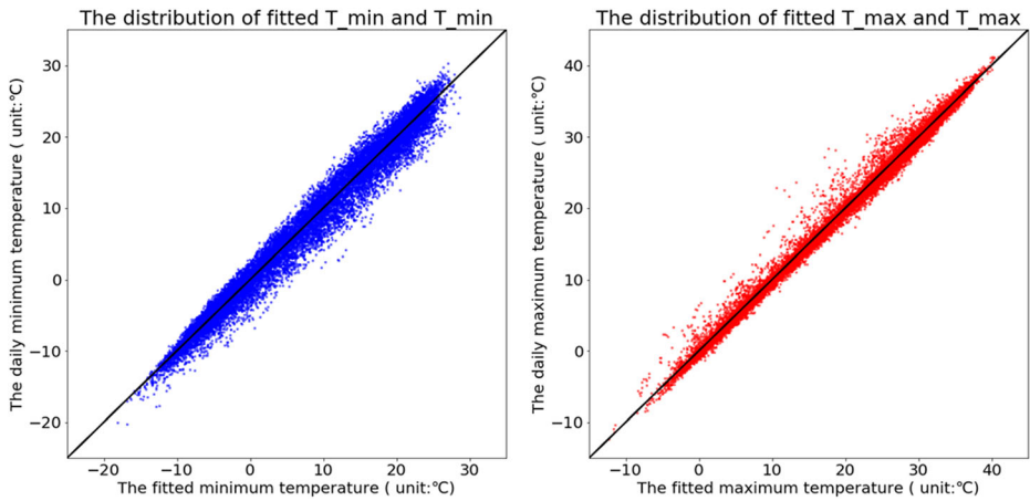
Fig. 5 The correlations of the fitted and observed daily T-min (left) and daily T-max (right) at the four national stations in Beijing urban area (unit: °C)
