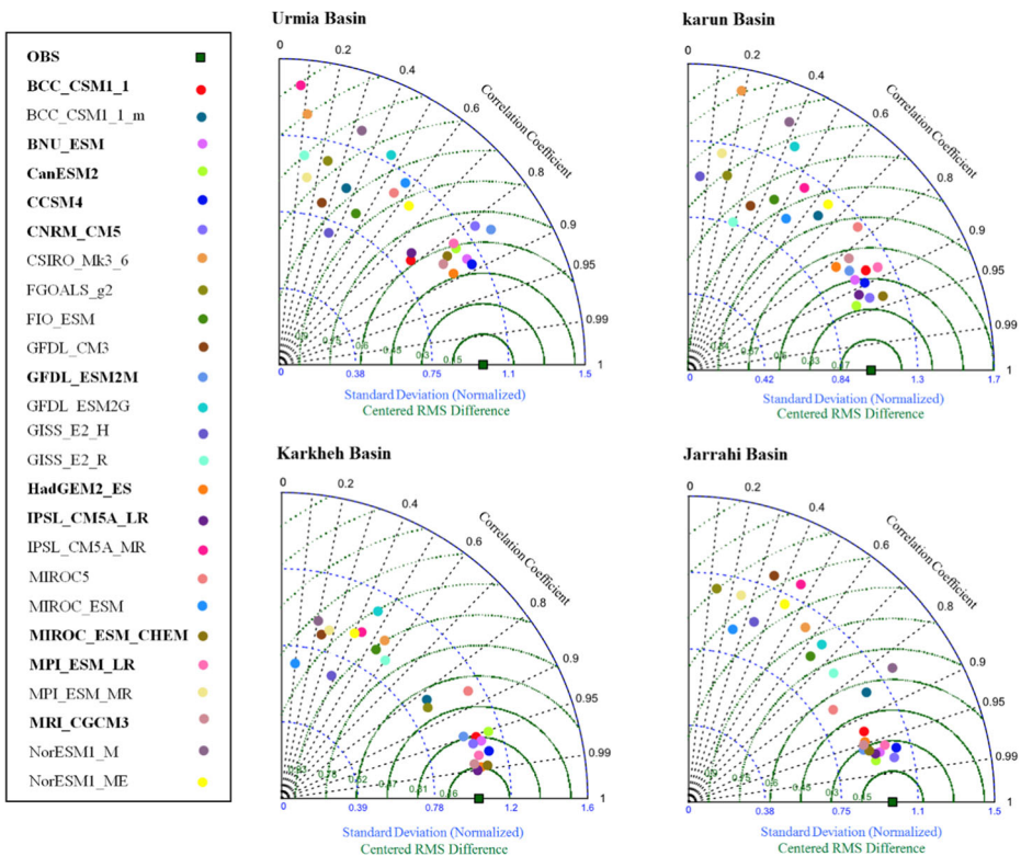
Fig. 2 Taylor diagrams comparing simulated precipitation from 25 GCMs against ground-based observations (1976–2005) in four selected basins. This diagram summarizes the correlation coefficient (dashed black lines), the ratio of the standard deviations (blue curves), and the RMSE (green curves). The closer the points to the observations (squares in x axes), the better is the agreement between simulations and observation
