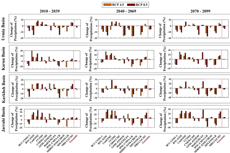
Fig. 3 Percent change (%) in projected precipitation in early, middle, and end of the twenty-first century relative to base period (1976–2005) based on best GCM simulations (individually and their ensemble mean) under two RCPs in the four selected basins in Iran
