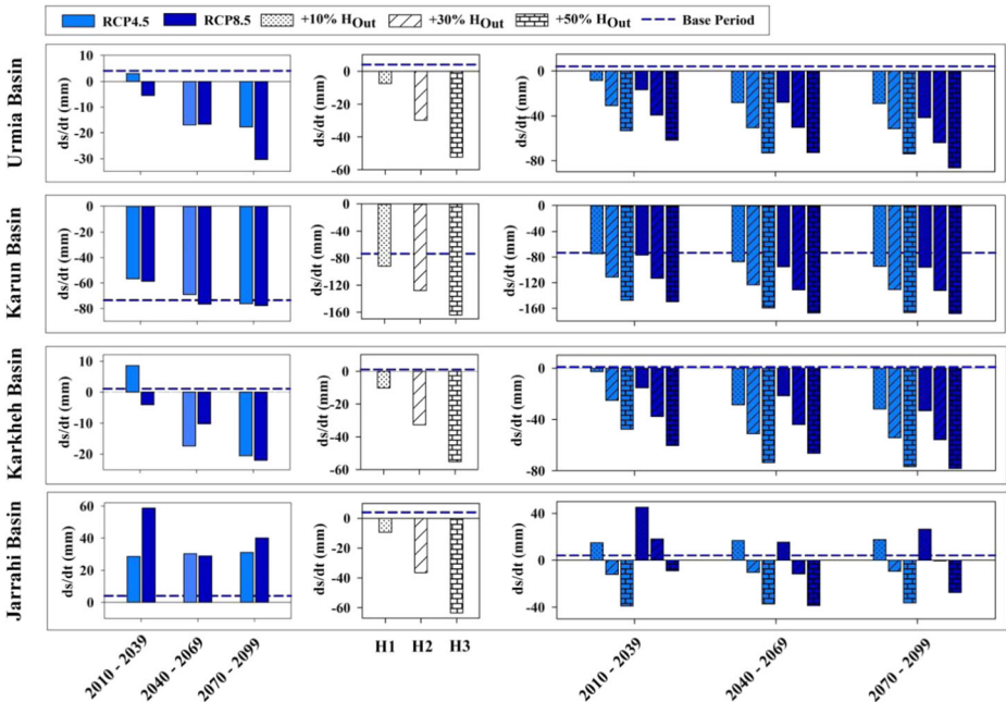
Fig. 4 Changes in basin storage ( ds/dt ) in early, middle and end of the twenty-first century relative to the baseline period (1976–2005) based on the ensemble mean of GCMs simulations and two RCPs (left panels), three water withdrawals scenarios (middle panels), and their compounding effects (right panels) in the four selected basins in Iran
