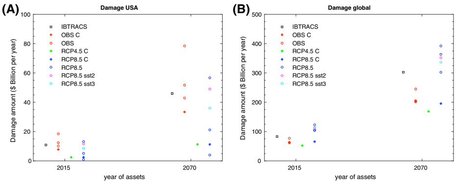
Fig. 3 a US and b global annual mean cyclone damage estimates for 2015 (left) and 2070 assets (right) for different CLIMADA simulations. Legend indicates CAM simulations: asterisks “c” are 1° coupling, open circles are 0.25° coupling simulations. Damage from observed (IBTRACS) storms as a black square. Different time periods are indicated by horizontal offsets (columns): IBTRACS on the left, then OBS (present day), RCP4.5 center and RCP8.5 climates right side of each time label
