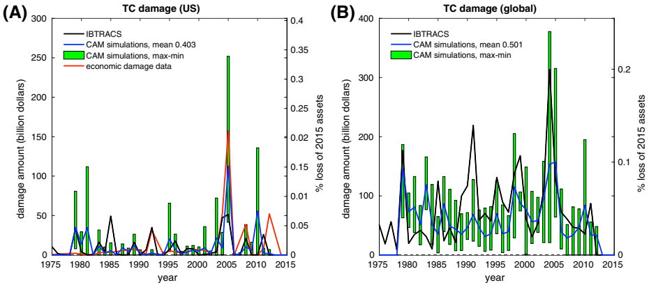
Fig. 2 Time series of annual loss from actual economic loss data (red lines), CAM simulation damage (blue line), range across CAM simulations (green bars) and IBTRACS (black line) for a US and b global. Similar to Fig. 1 but for damage in billion USD (left scale) and percent loss (right scale). Correlations printed between mean CAM and IBTRACS
