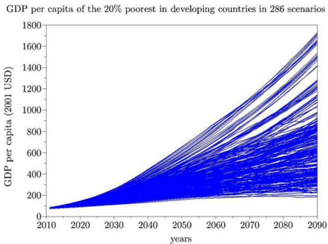
Fig. 2 GDP per capita of the 20 % poorest in a selection of developing countries in 286 scenarios resulting from 143 model runs with IMACLIM-R and two hypotheses on the share of income of the 20 % poorest
