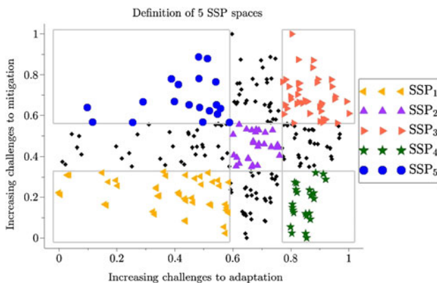
Fig. 3 Capacities to adapt and to mitigate that define the five SSP spaces and the results of our 286 model runs arrayed in this space
