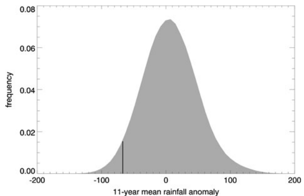
Fig. 4 Histogram of all 11-year mean rainfall anomalies generated from the 10,000-member rainfall reconstruction (1783–1988) and AWAP rainfall observations (1900–2009). The solid vertical line indicates the 1998–2008 decadal rainfall anomaly in relation to the full reconstruction ensemble
