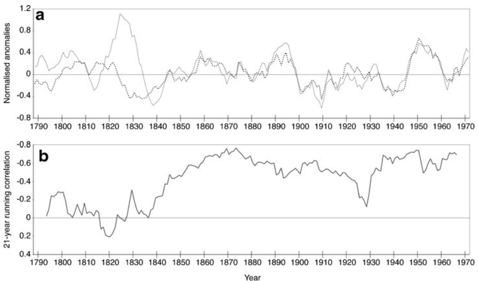
Fig. 5 a 11-year running means of the SEA rainfall reconstruction (the ensemble median, shown by the solid line) and the Unified ENSO Proxy (dashed line) from 1788–1971. Note that the UEP has been inverted and lagged by one year for comparison with the SEA rainfall reconstruction and anomalies are relative to a common 1900–1976 base period. b 21-year running correlation of the inter-annual variations of the SEA rainfall reconstruction and the UEP, 1793–1966. Note that the y-axis has been inverted
