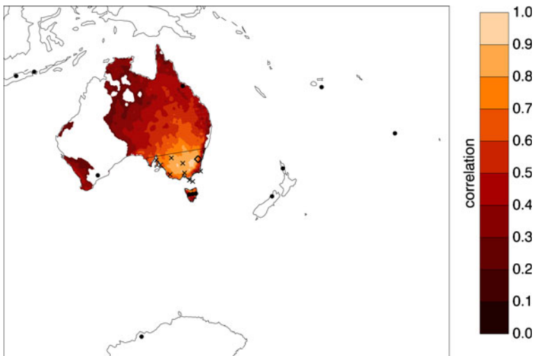
Fig. 1 Correlations between annual variations in May–April southeast Australia area-averaged rainfall and point rainfall on the Australian continent. The boundary of southeast Australia as defined in this study is outlined in black. The locations of the proxy data ( solid circles ), the high-quality station data ( crosses ) and the location of Lake George ( open diamond ) are shown
