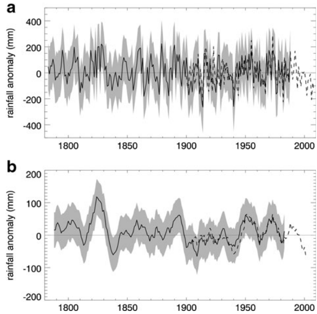
Fig. 3 The SEA rainfall reconstruction from 1783–1988 at a inter-annual and b decadal time-scales. The solid black line represents the median of the distribution of 10,000 rainfall reconstructions. The grey shading indicates \pm two standard deviations of the error distribution, calculated as the combined errors between the reconstruction ensemble members and the observations associated with the calibration period and the random errors associated with ‘climate noise’. The dashed line shows the instrumental AWAP rainfall data used for 20th century calibration and verification (1900–1988)
