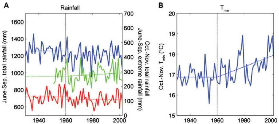
Fig. 1 Historical weather observations for a representative kharif rice-growing region in predominantly rainfed areas of India. Observations were constructed by weighting state-level weather variables by 1966–2002 mean areas harvested. Dotted lines show trends. a Total June–Sep. rainfall ( blue , left axis); total Oct.–Nov. rainfall ( red , right axis); June–Sep. extreme rainfall ( green , right axis). b Oct.–Nov. T_{\min}
