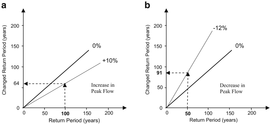
Fig. 4 Examples of how the fluvial model works: a The effect of an increase of 10% peak flow on the frequency of fluvial flooding. The one in 100 year event became a one in 64 year event. b How the model works in reverse in order to allow more flow capacity within the river channel by raising the height of river defences. The one in 50 standard of protection became one in 91
