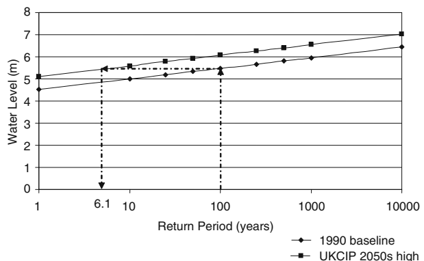
Fig. 3 An example of the flood probability curves in North Norfolk showing the 1990 baseline and the effect of the 2050s high sea-level rise scenario (i.e. 54 cm). The one in 100 year event is degraded to one in 6.1 year event
