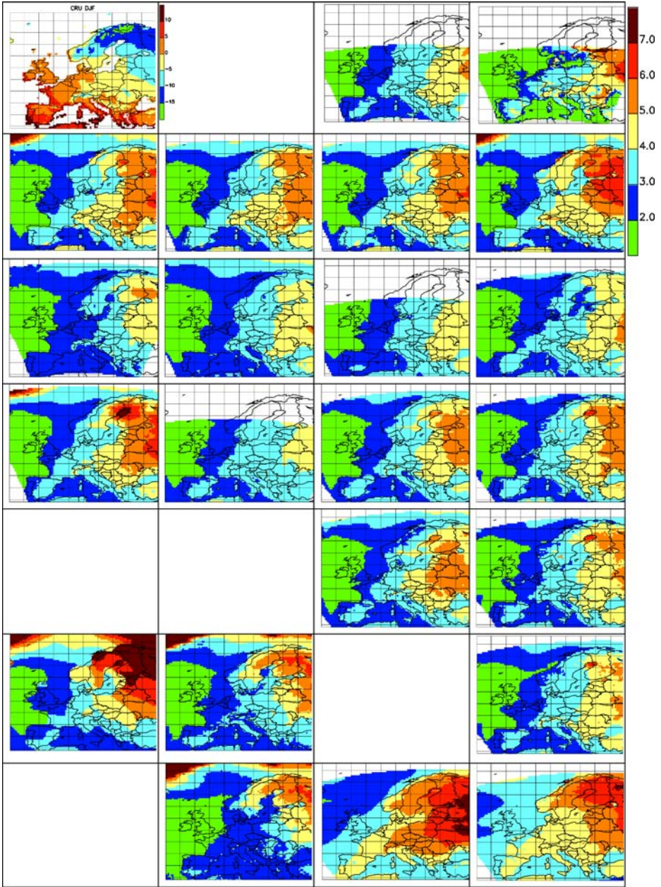
Fig. 2 a Temperature Change [°C] DJF, cf. Fig. 1. The standard deviation has been scaled by a factor of 10. b Temperature Change [°C] JJA, cf. Fig. 1. The standard deviation has been scaled by a factor of 10
