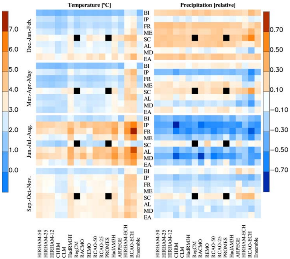
Fig. 5 A schematic overview of seasonal changes as simulated by the PRUDENCE regional models. In each panel, rows are the analysis areas, columns correspond to models. Rows of panels signify the four seasons, the left column of panels are temperature change (left color bar, degrees C), whereas the right column of panels signifies precipitation (right color bar, relative change). Areas not covered by a particular model are indicated by black squares
