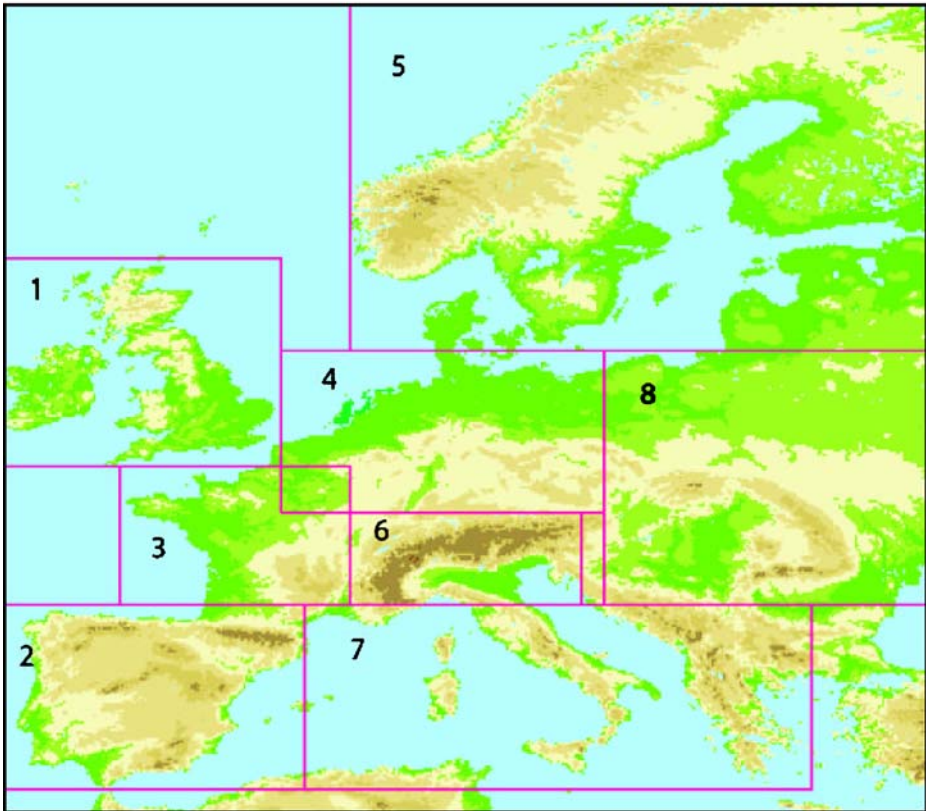
Fig. 4 European sub-areas
