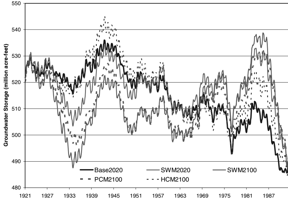
Figure 5. Groundwater storage over the 72-year period at 2100 water demand levels.
