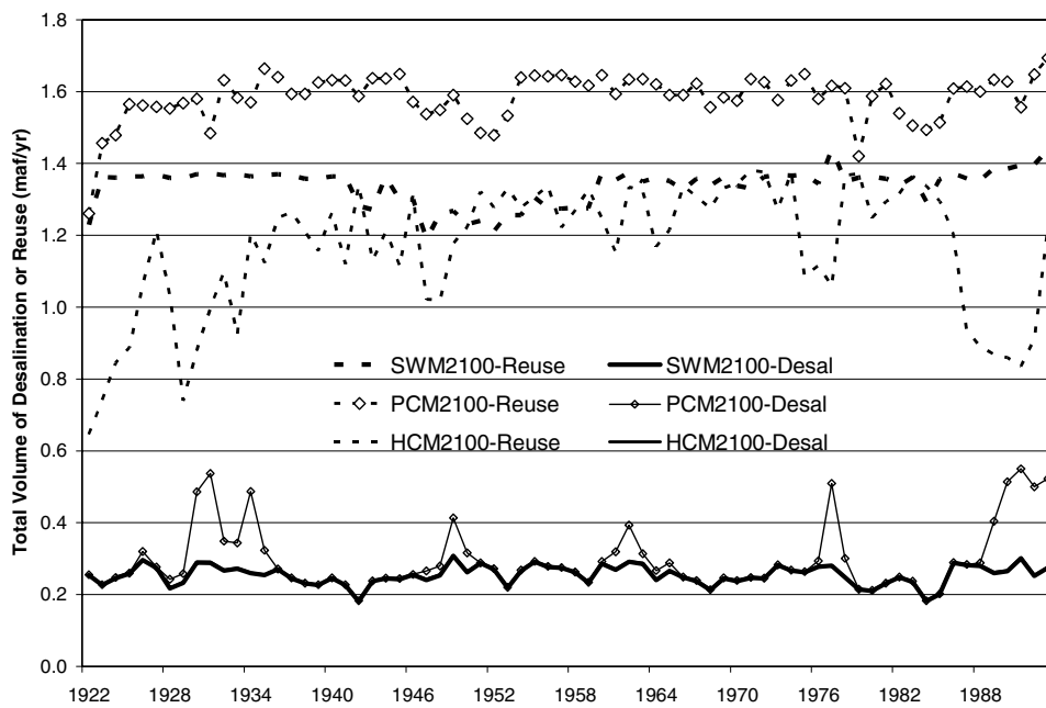
Figure 8. Use of seawater desalination and urban wastewater recycling at 2100 water demand levels.
