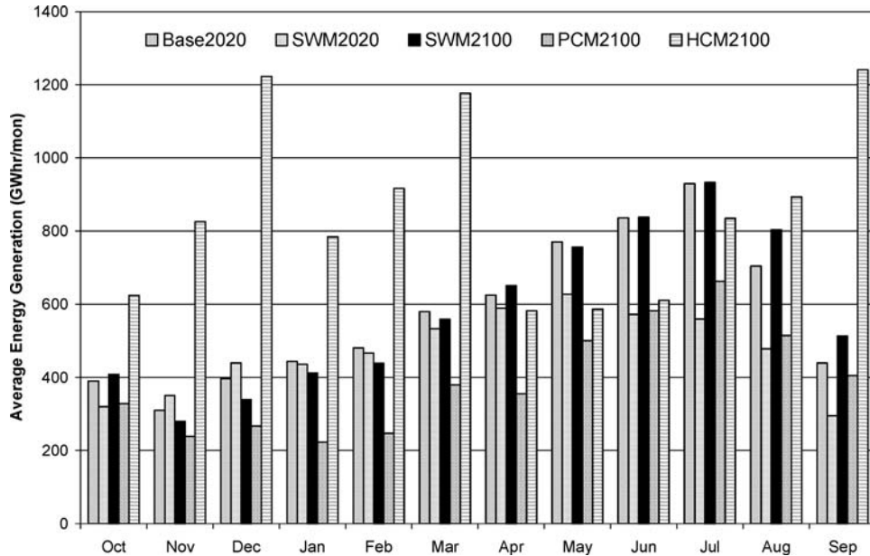
Figure 10. Average seasonal hydropower generation from major reservoirs.
