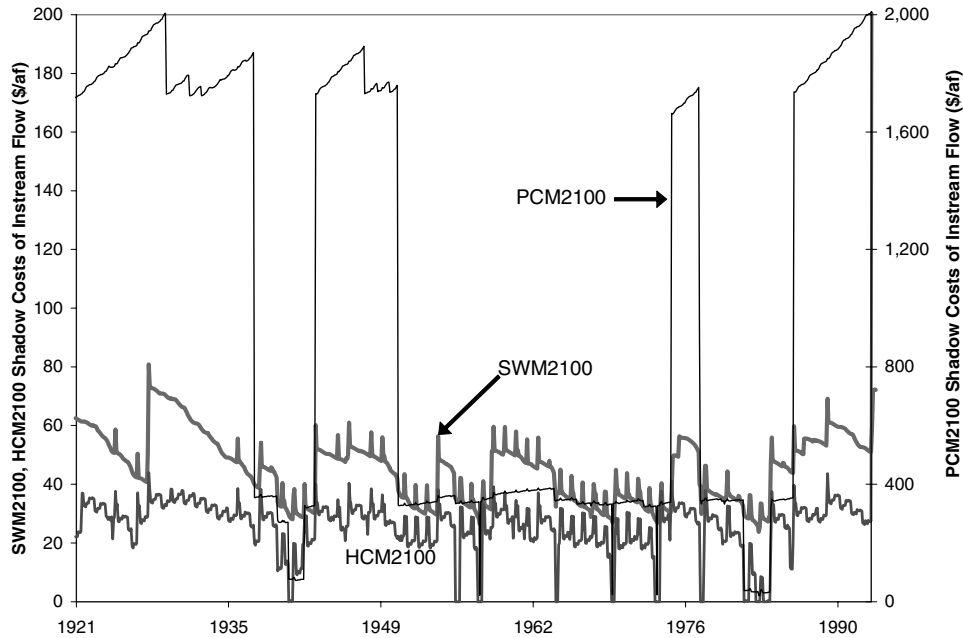
Figure 9. Time series of shadow costs for trinity river instream flow requirement.
